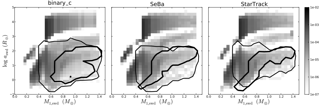
Fig. A.8. Orbital separation versus WD mass for all SWDs in the full mass range at the time of SWD formation. The contours represent the SWD population from a specific channel: channel 2a (thin line) and channel 2b (thick line).
