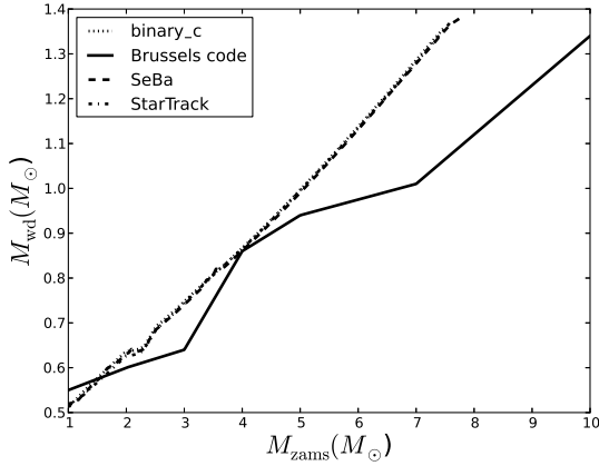
Fig. 7. Initial-final mass relation of single stars that become WDs for the different groups, dotted line shows the results of binary_c , solid line the results of the Brussels code, the dashed line the results of SeBa , and the dash-dotted line the results of StarTrack .
