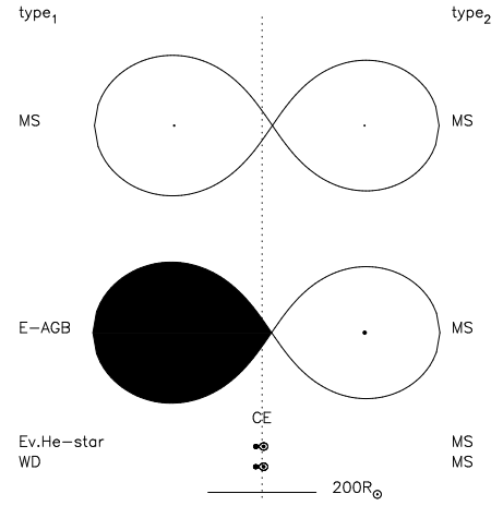
Fig. A.7. Example of the evolution of a SWD system in channel 2a. Abbreviations are as in Table A.2.
