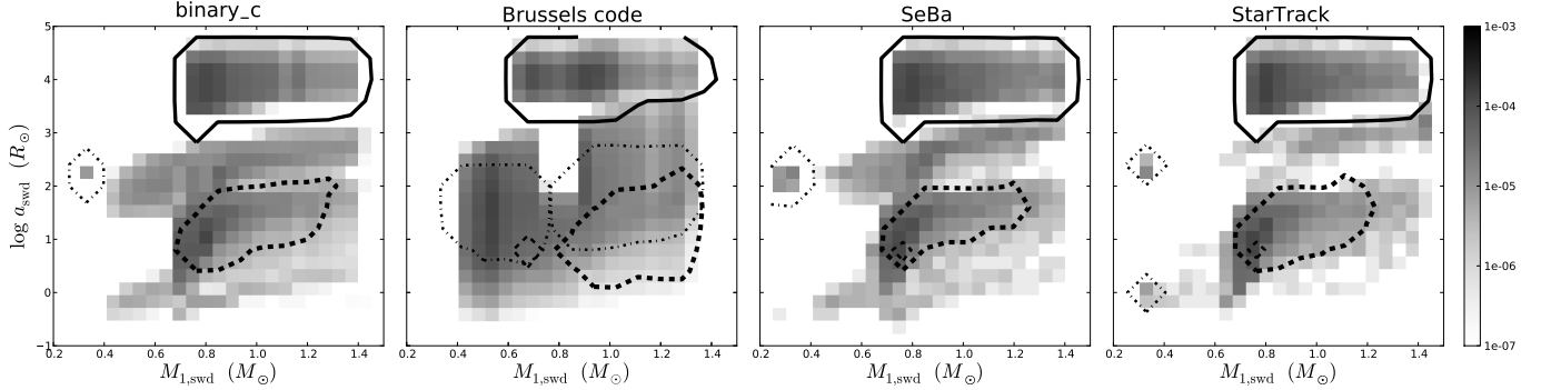
Fig. A.2. Orbital separation versus WD mass for all SWDs in the intermediate mass range at the time of SWD formation. The contours represent the SWD population from a specific channel: channel 1 (solid line), channel 4a (thin dashed line), channel 4b (thick dashed line) and channel 5 (dash-dotted line).
