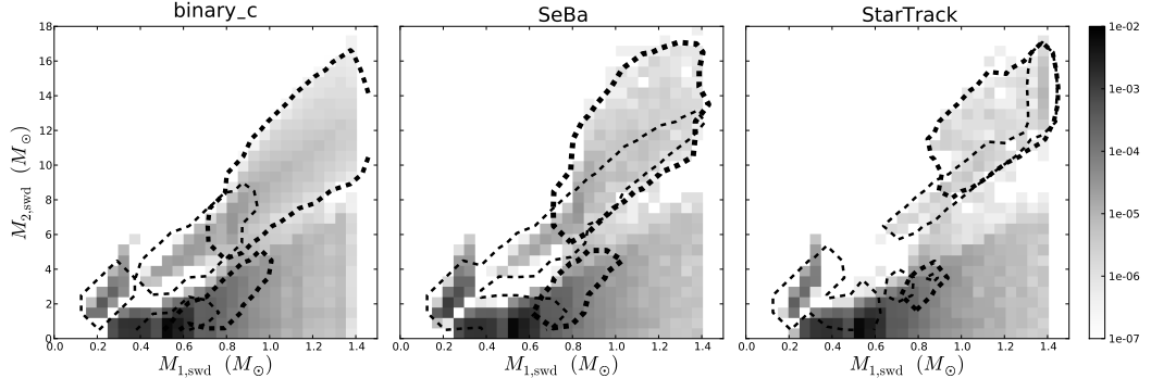
Fig. A.17. Secondary mass versus WD mass for all SWDs in the full mass range at the time of SWD formation. The contours represent the SWD population from a specific channel: channel 3a (thin line) and channel 3b (thick line).
