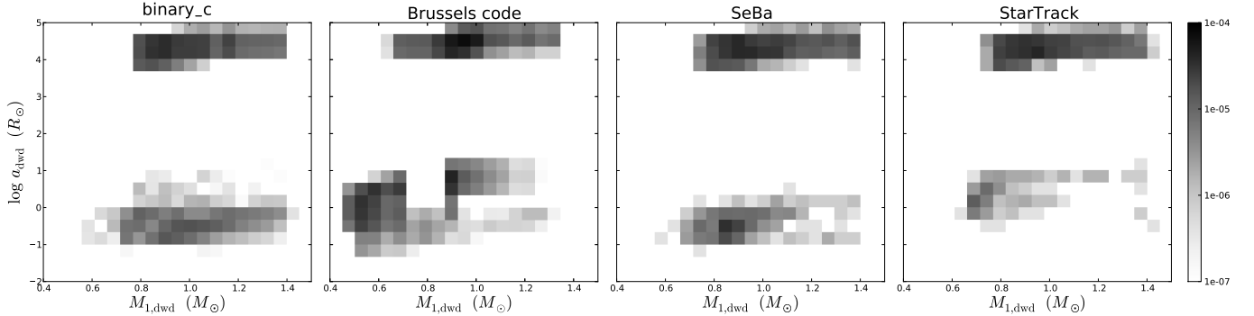
Fig. 9. Orbital separation versus primary WD mass for all DWDs in the intermediate mass range at the time of DWD formation.
