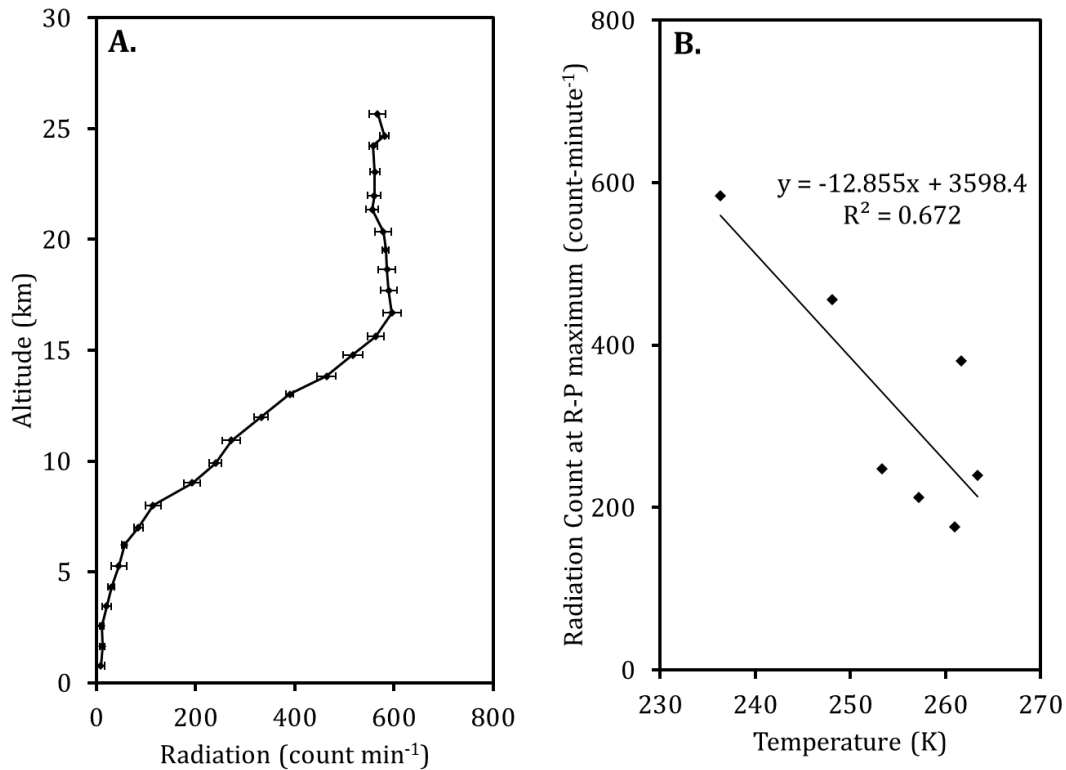
Fig. 2 (A.) Radiation profile measured by on-board Geiger counter. (B.) relationship of Regener-Pfotzer (R-P) maximum with temperature
