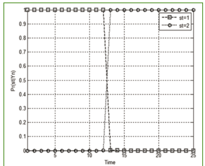
Figure 4. Pr(st=k|Yn) , Germplasm demand dataset. Source: Author’s calculations
