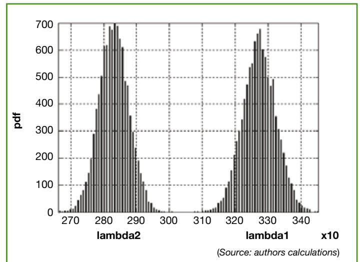
Figure 3. Posterior marginal densities of \lambda_1 and \lambda_2 .
