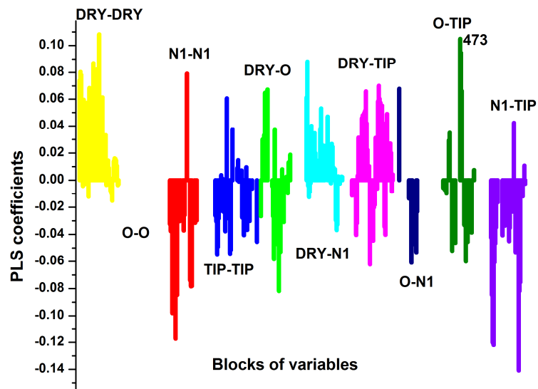
Figure 2. PLS coefficients plot, obtained with 3LV.
