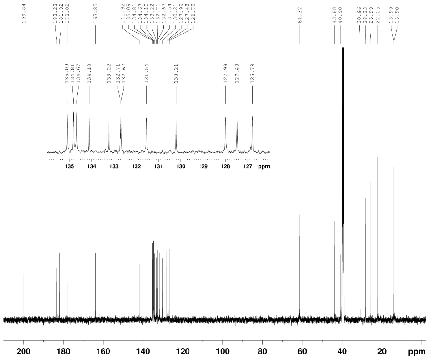
Fig. S18. ^{13}\text{C} NMR spectrum of 5c .
