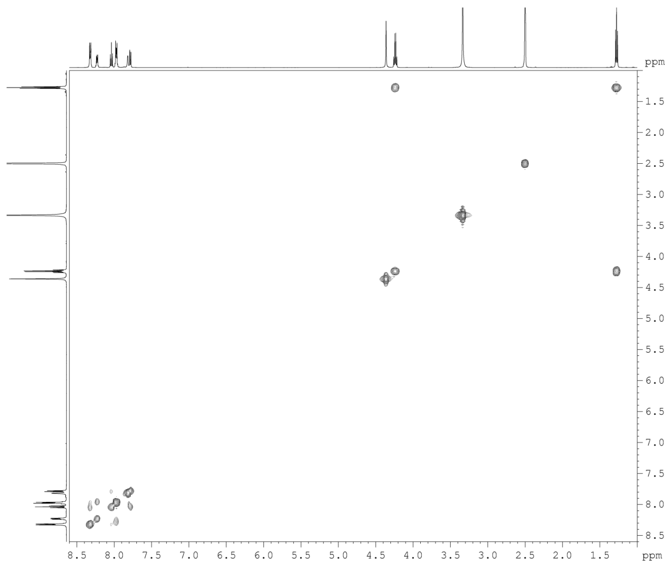
Fig. S8. COSY spectrum of 5a .
