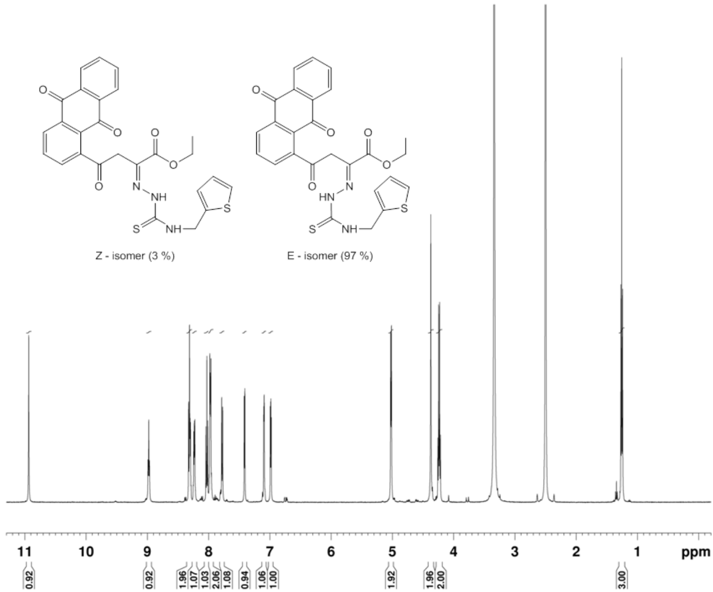
Fig. S25. 1 H NMR spectrum of 5f.
