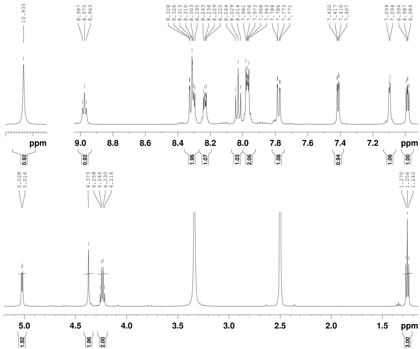
Fig. S26. Expanded ^1\text{H} NMR spectrum of 5f .
