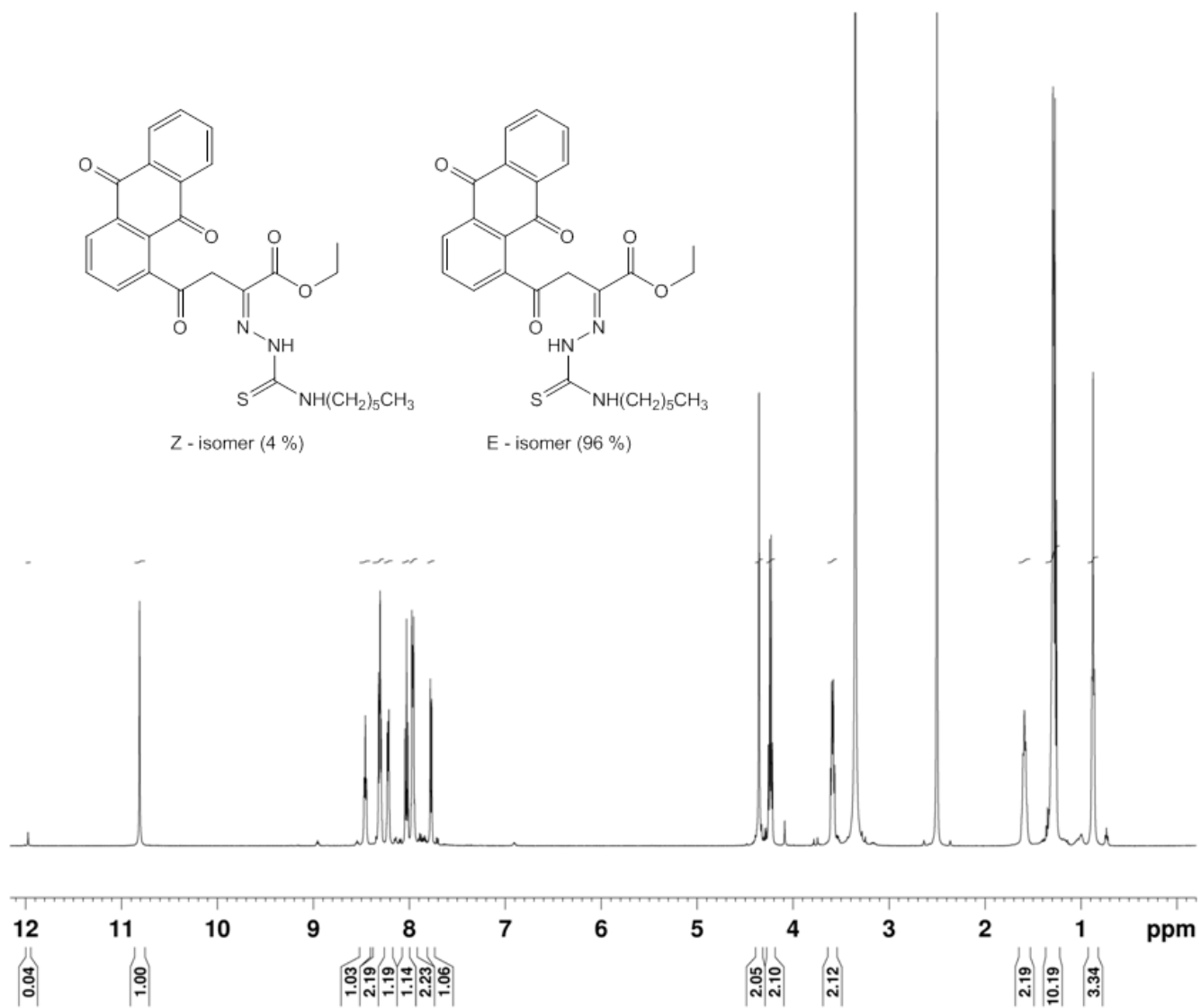
Fig. S16. 1 H NMR spectrum of 5c.
