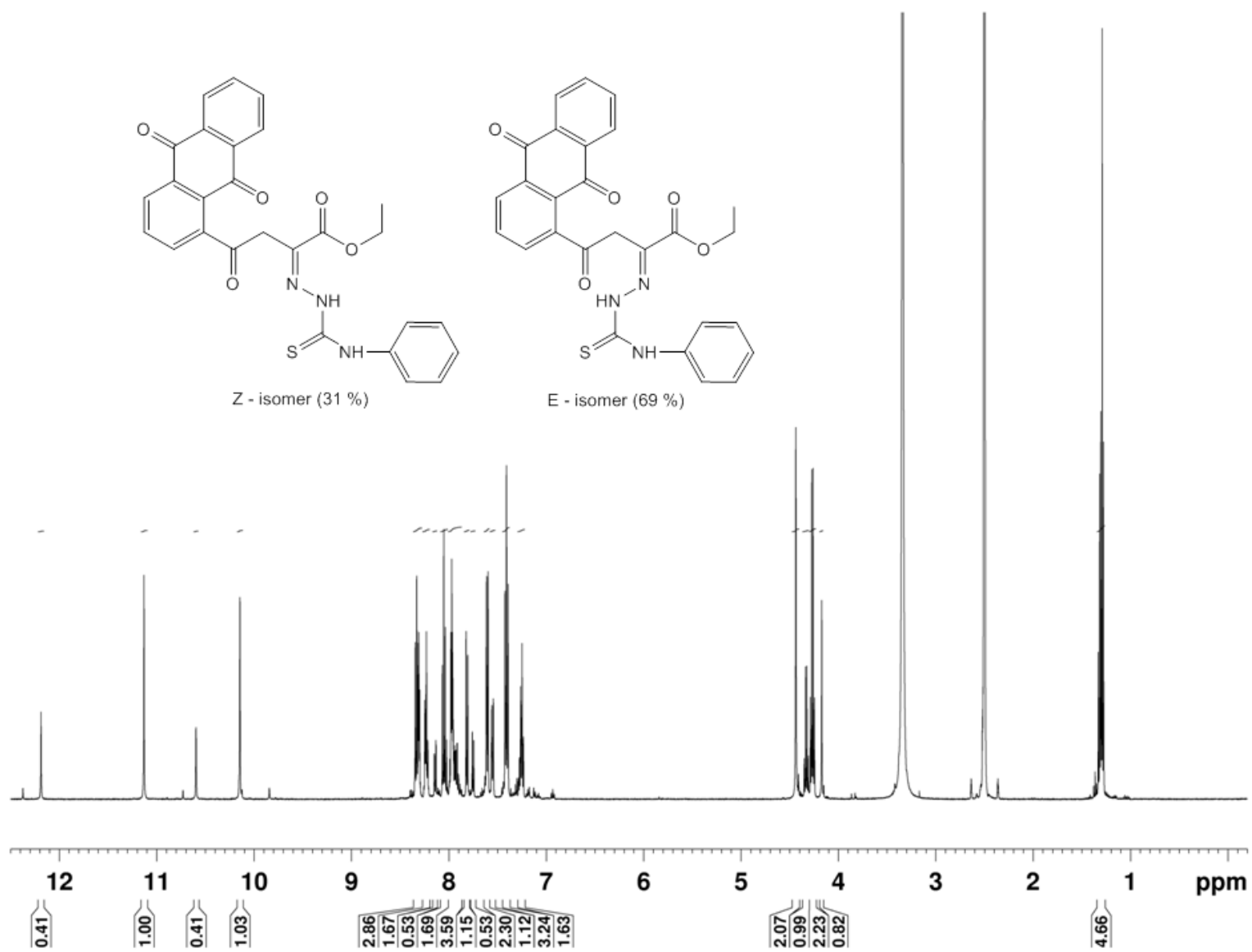
Fig. S31. 1 H NMR spectrum of 5h.
