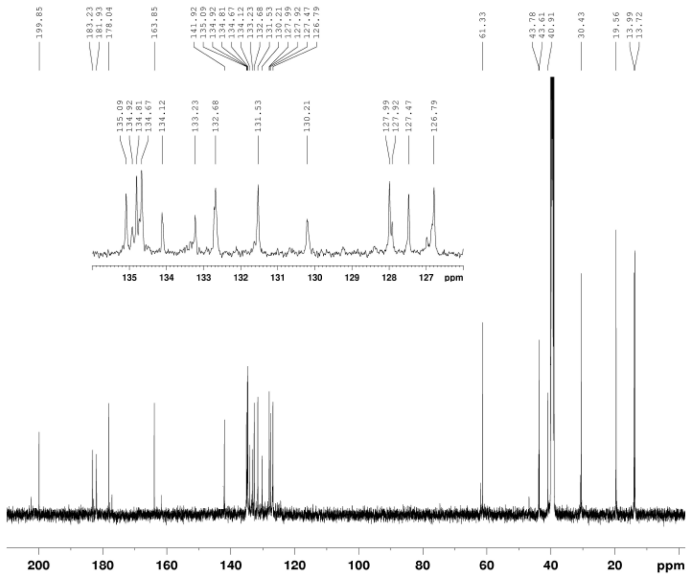
Fig. S15. ^{13}\text{C} NMR spectrum of 5b .
