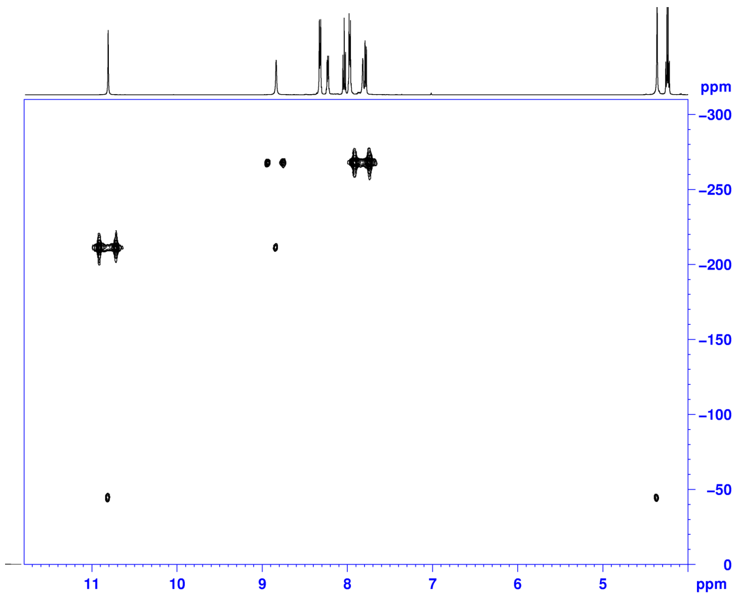
Fig. S12. ^1\text{H} - ^{15}\text{N} HMBC spectrum of 5a .
