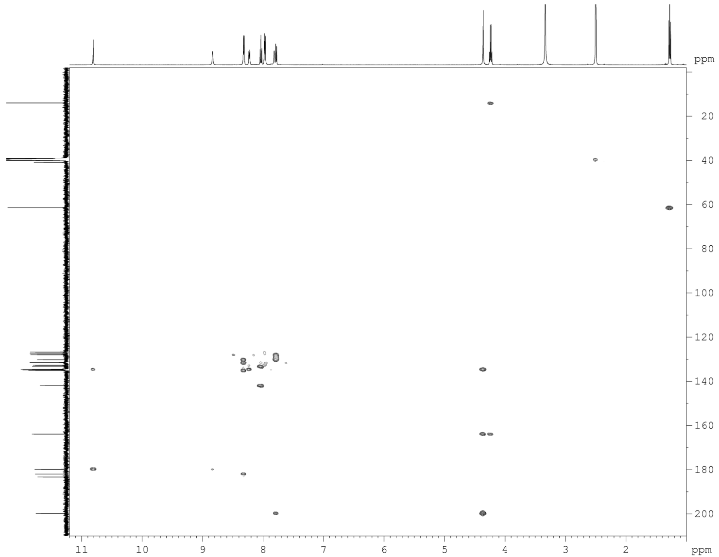
Fig. S10. HMBC spectrum of 5a .
