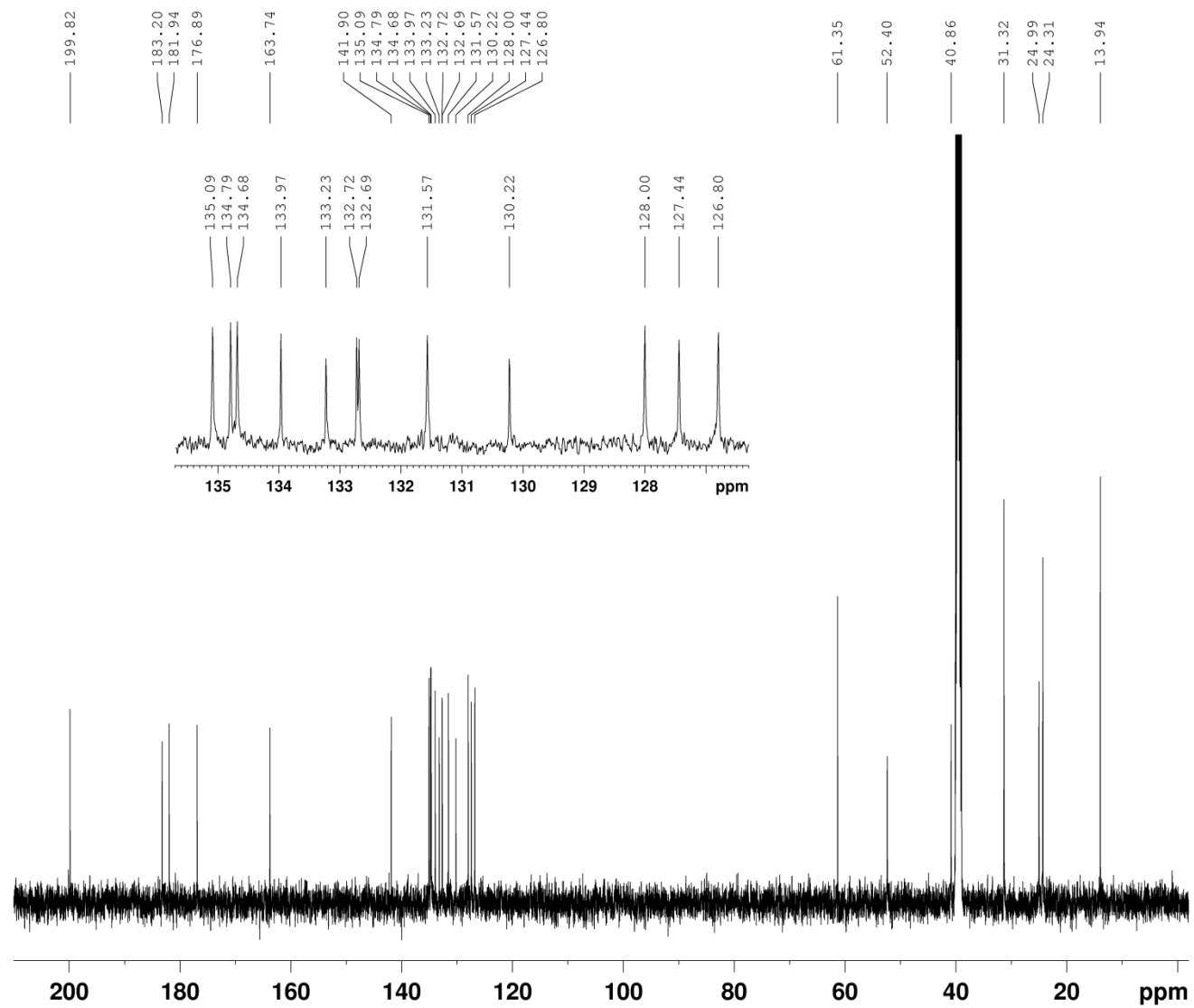
Fig. S21. ^{13}\text{C} NMR spectrum of 5d .
