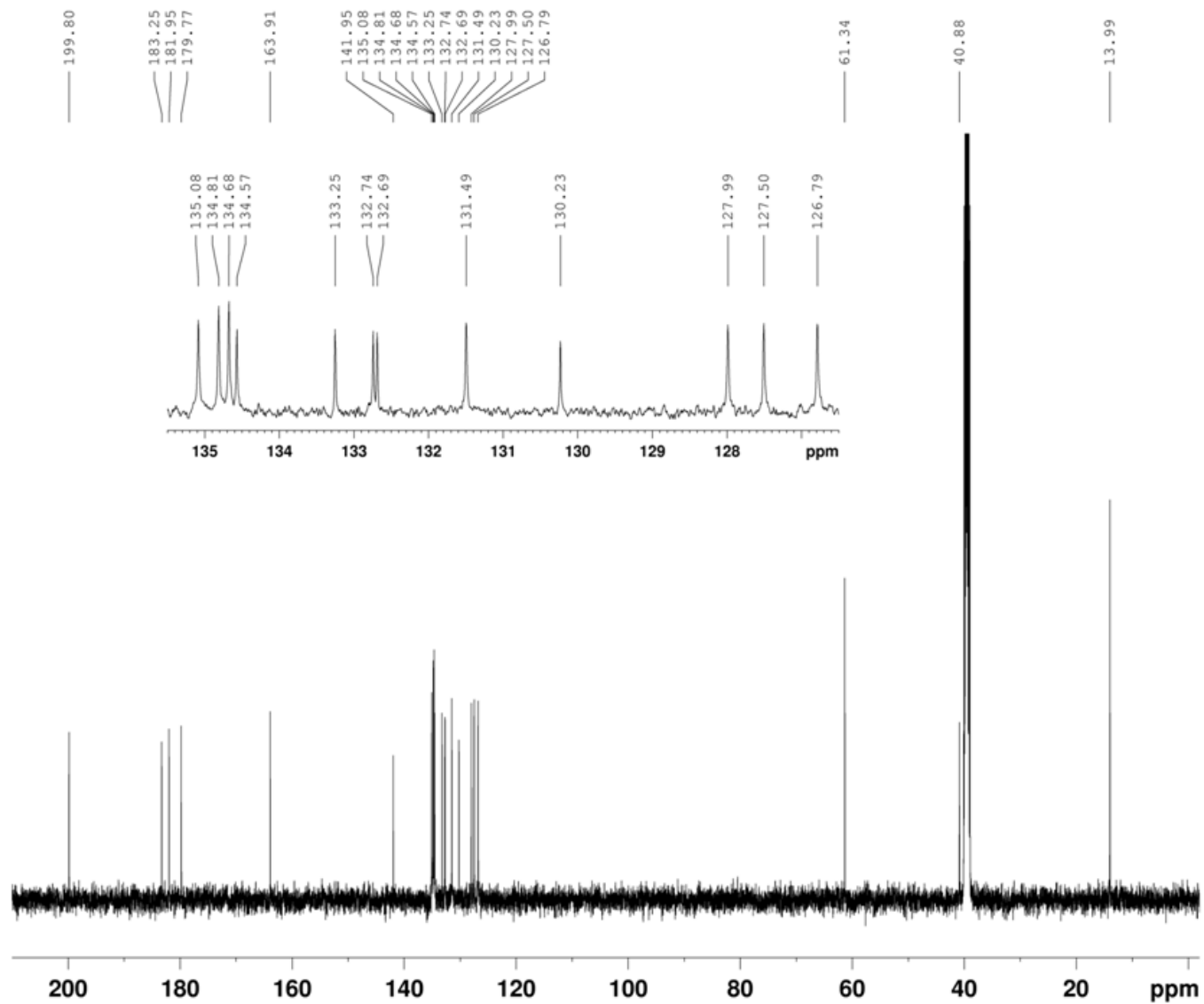
Fig. S6. ^{13}\text{C} NMR spectrum of 5a .
