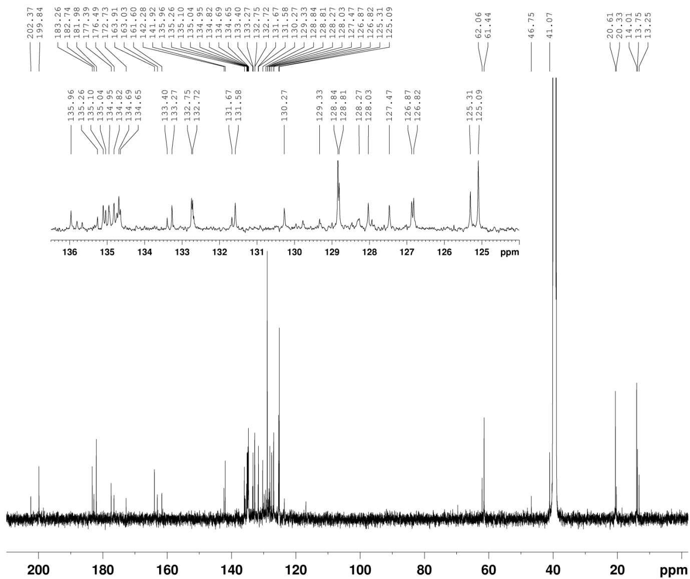
Fig. S36. ^{13}\text{C} NMR spectrum of 5i .
