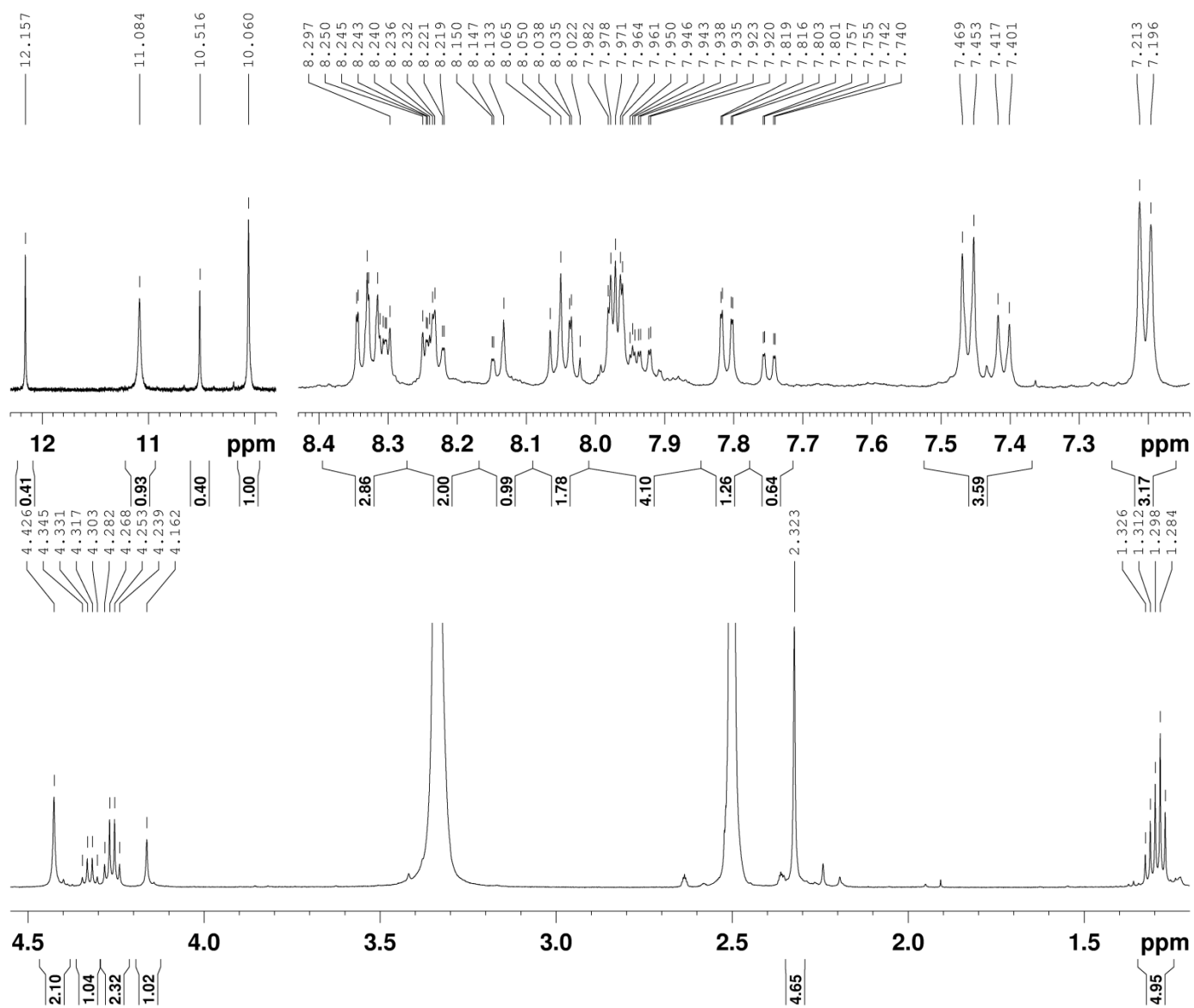
Fig. S35. Expanded ^1\text{H} NMR spectrum of 5i .
