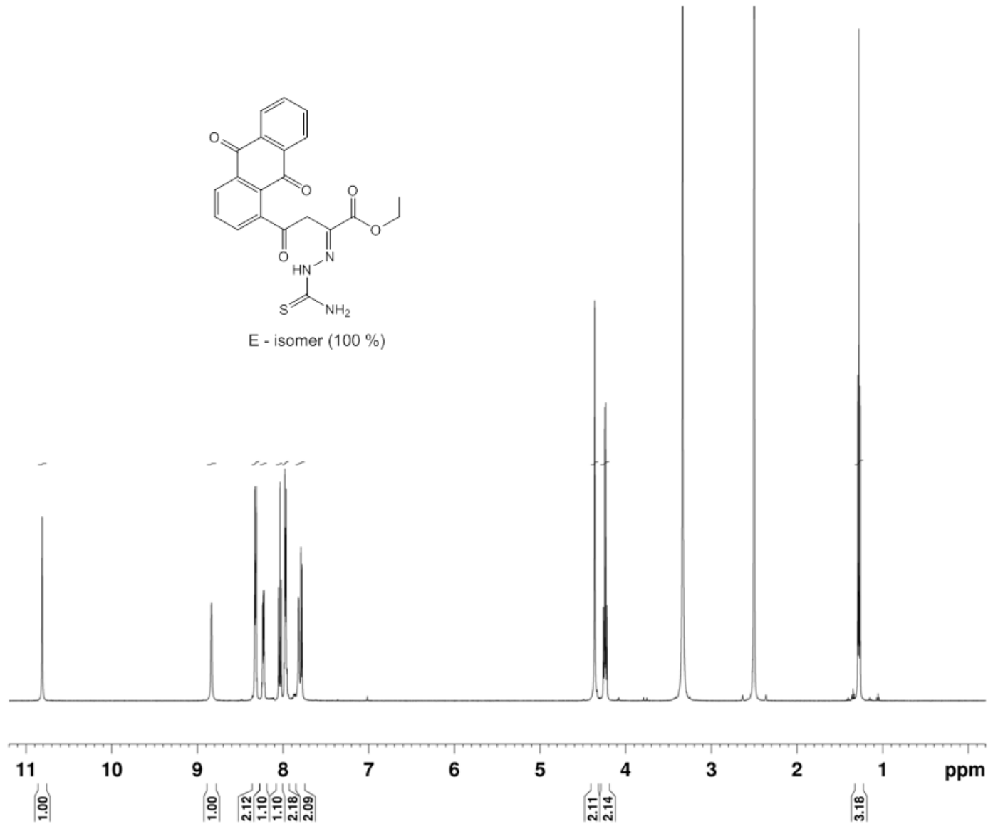
Fig. S4. 1 H NMR spectrum of 5a.
