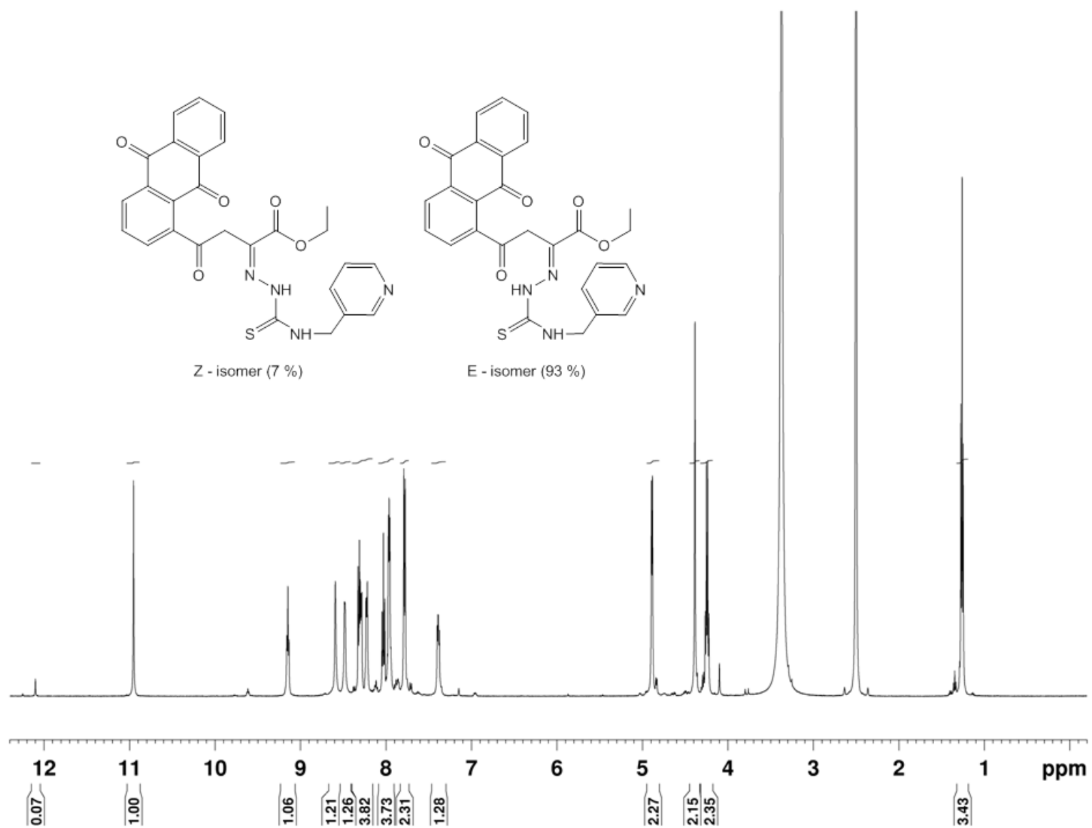
Fig. S28. 1 H NMR spectrum of 5g.
