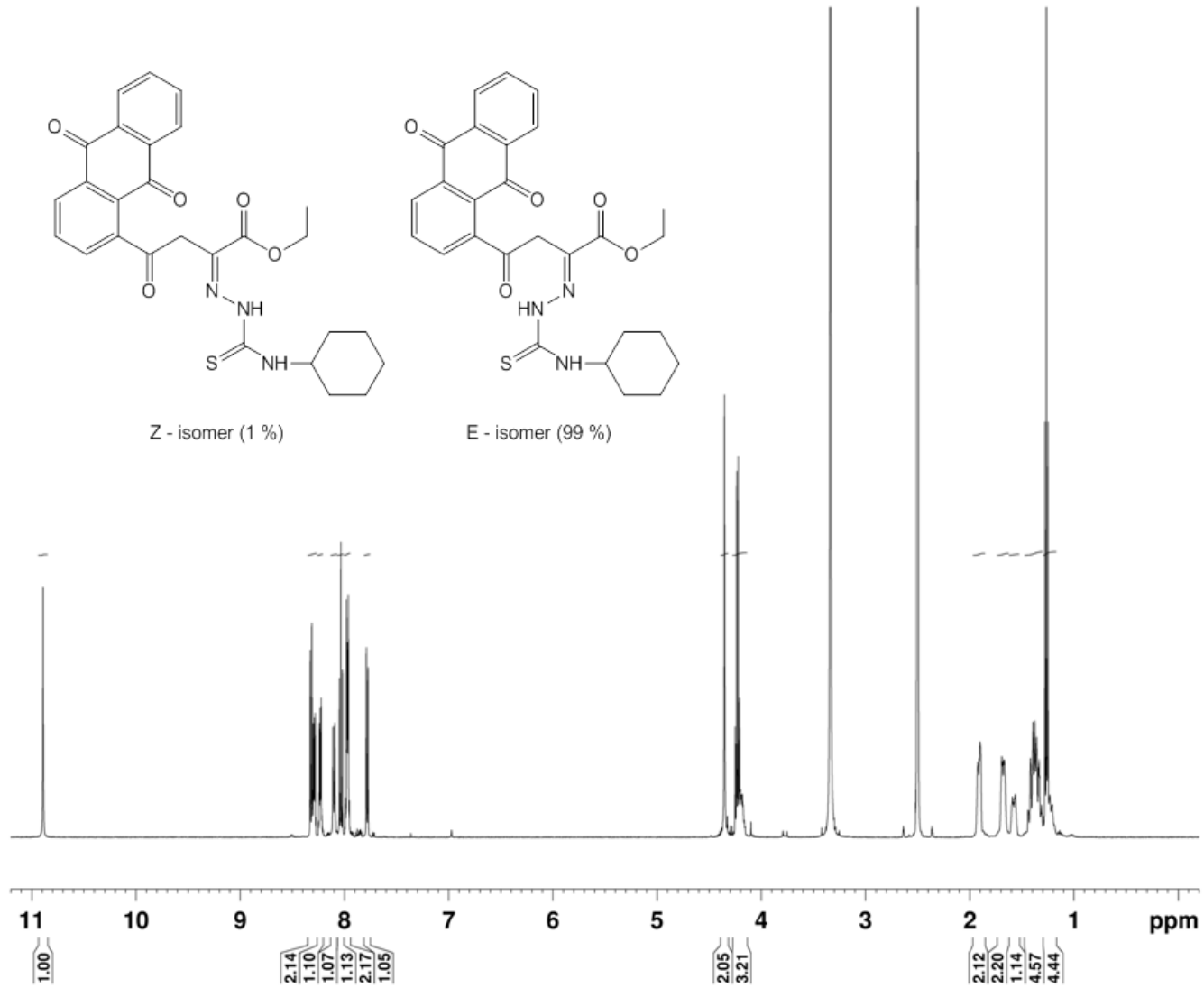
Fig. S19. 1 H NMR spectrum of 5d.
