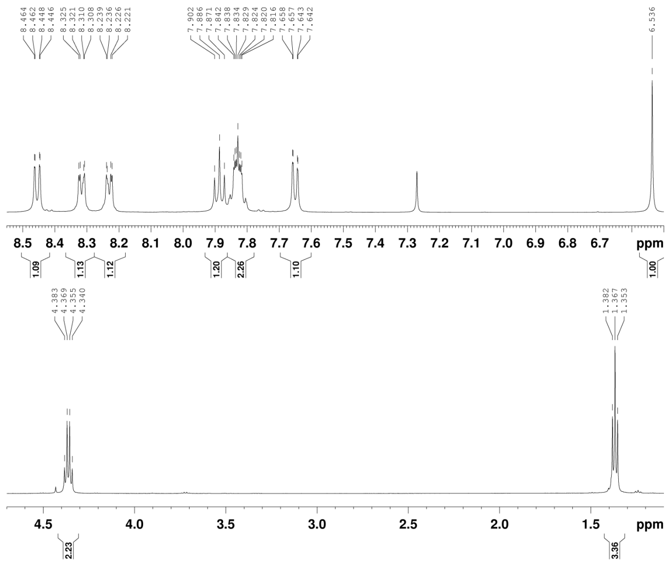
Fig. S2. Expanded ^1\text{H} NMR spectrum of 4 .
