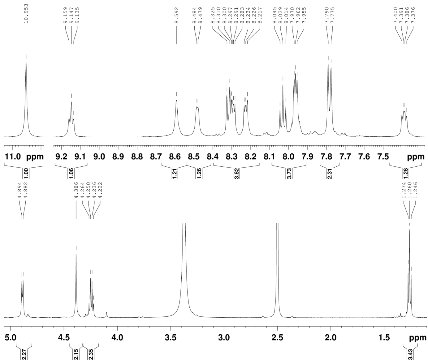
Fig. S29. Expanded ^1\text{H} NMR spectrum of 5g .
