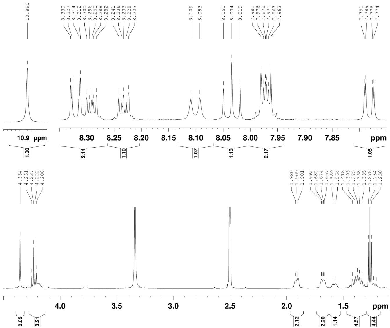
Fig. S20. Expanded ^1\text{H} NMR spectrum of 5d .
