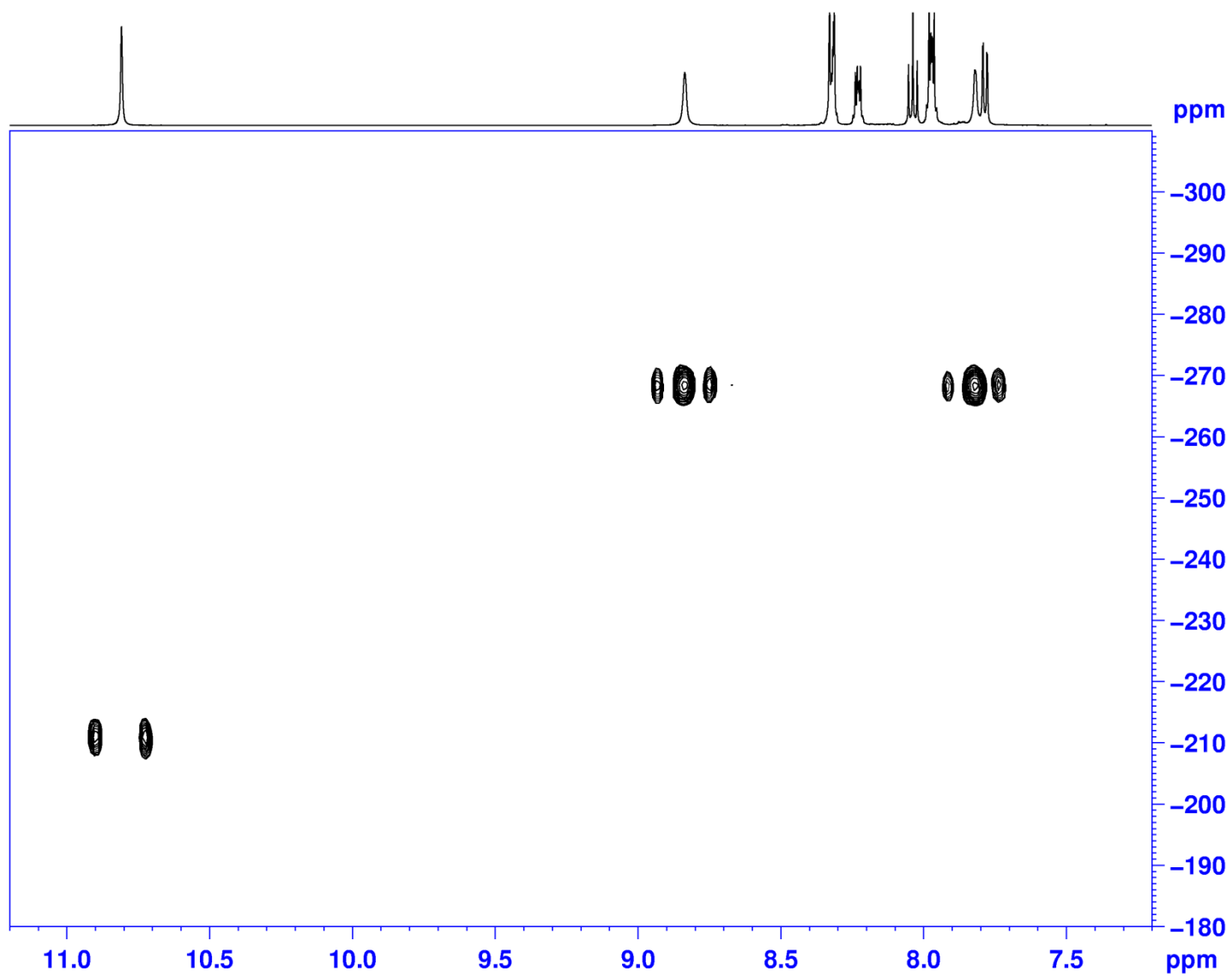
Fig. S11. ^1\text{H} - ^{15}\text{N} HSQC spectrum of 5a .
