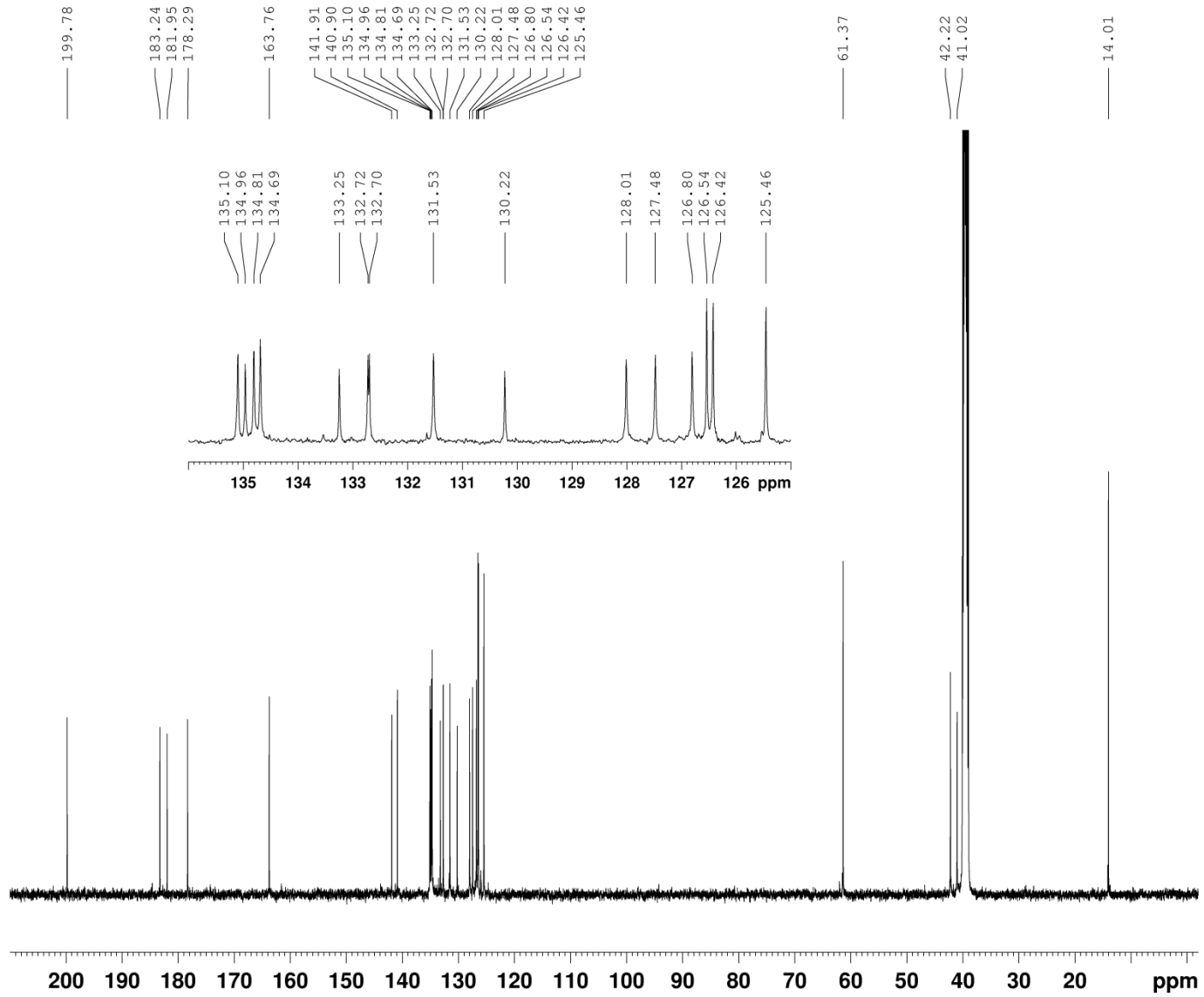
Fig. S27. ^{13}\text{C} NMR spectrum of 5f .
