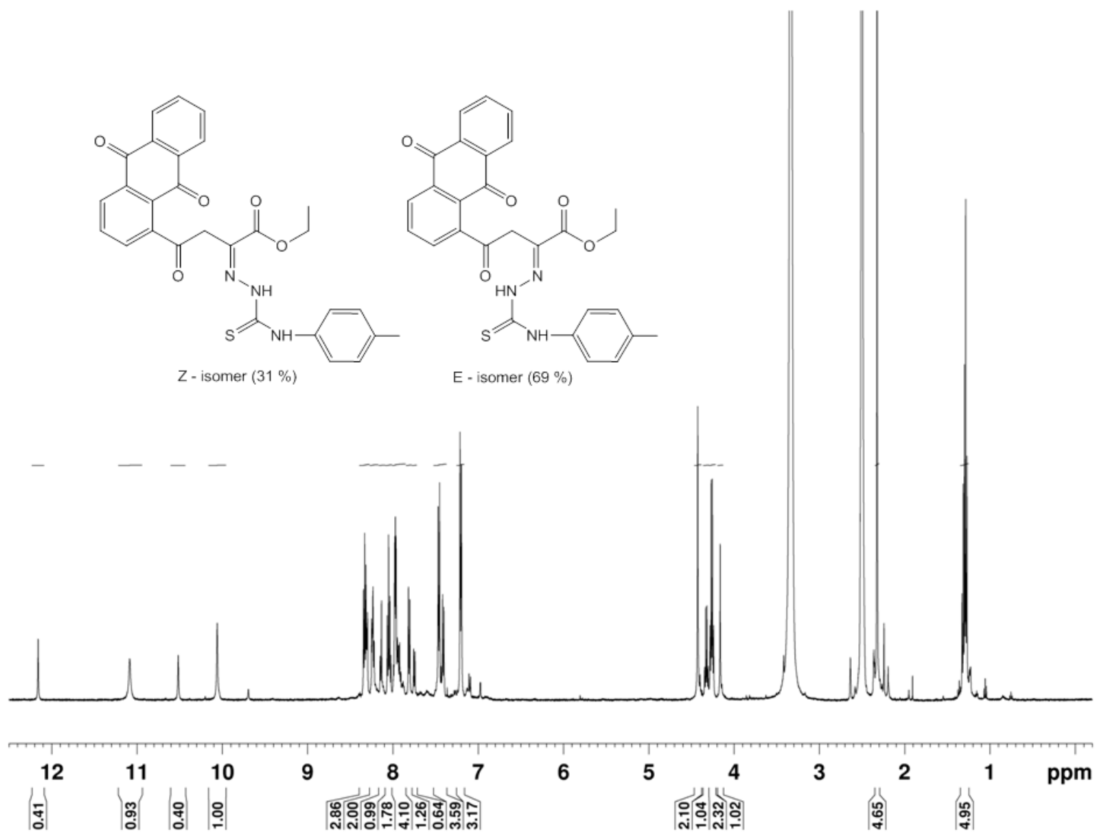
Fig. S34. 1 H NMR spectrum of 5i .
