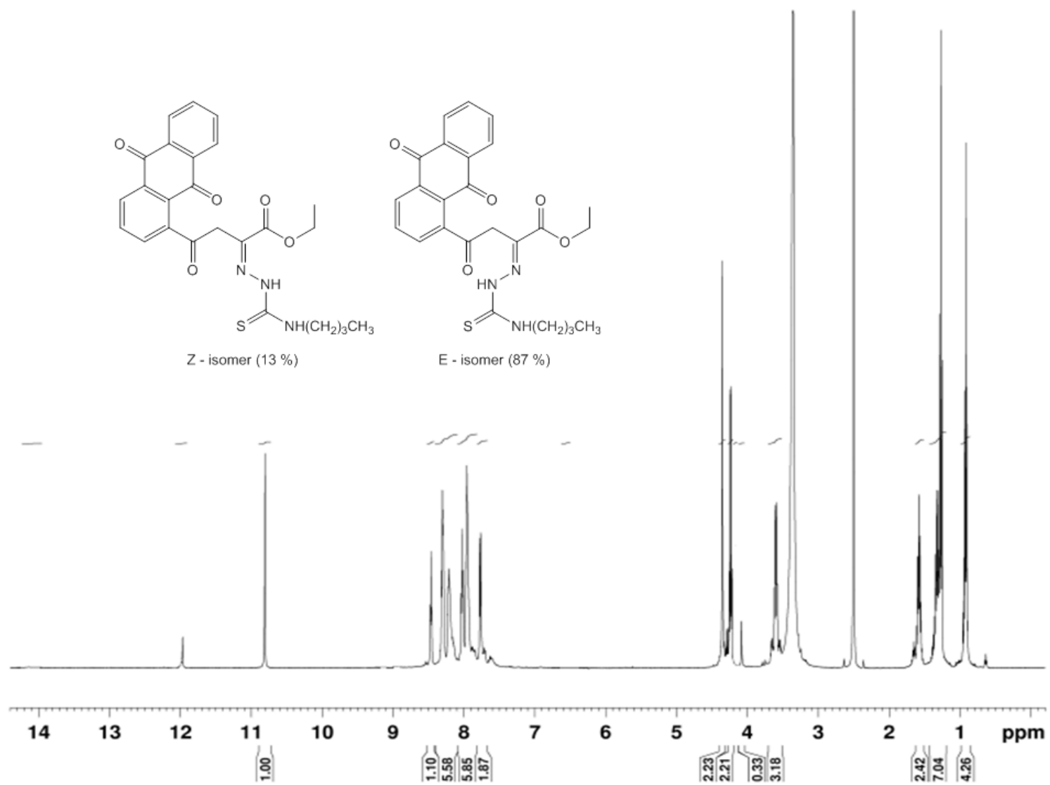
Fig. S13. 1 H NMR spectrum of 5b .
