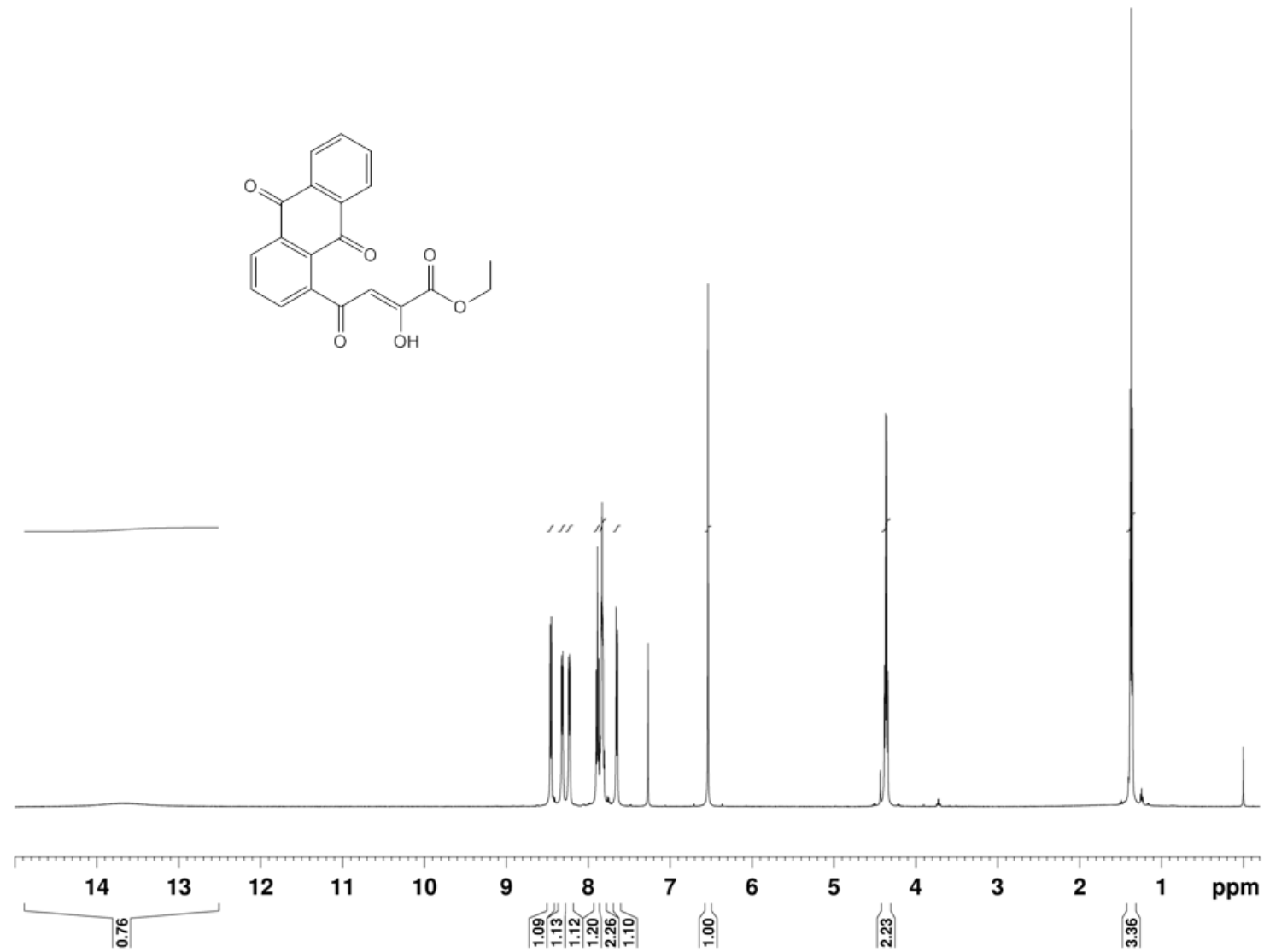
Fig. S1. 1 H NMR spectrum of 4.
