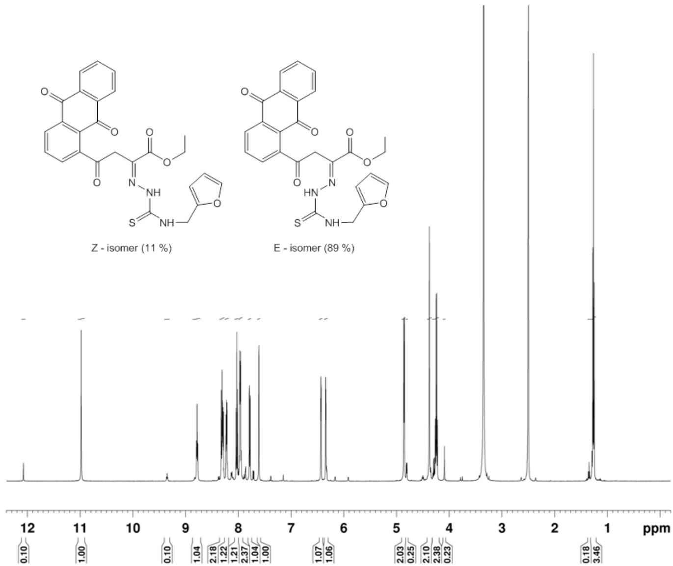
Fig. S22. 1 H NMR spectrum of 5e.
