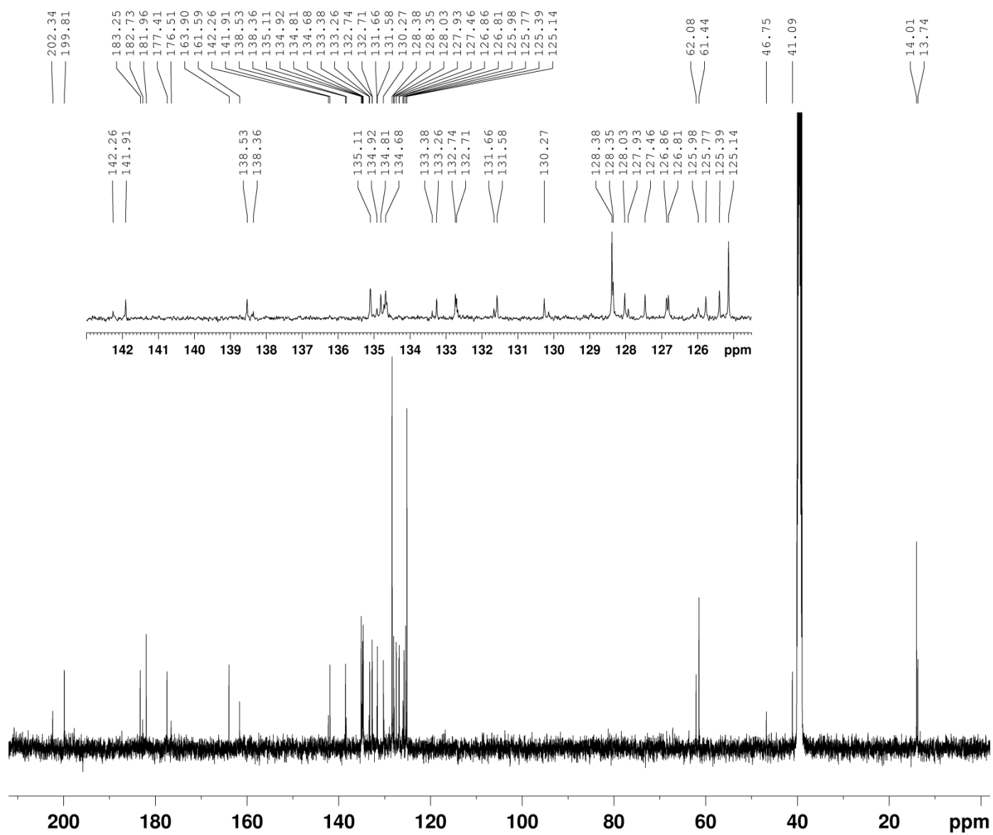
Fig. S33. ^{13}\text{C} NMR spectrum of 5h .
