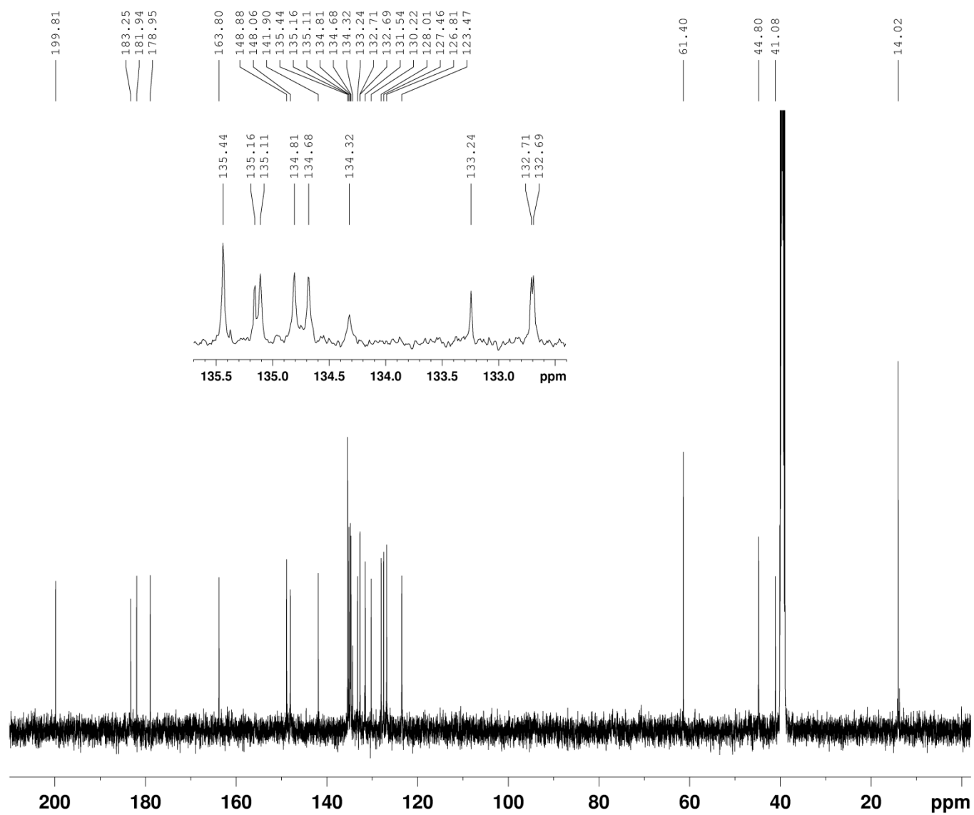
Fig. S30. ^{13}\text{C} NMR spectrum of 5g .
