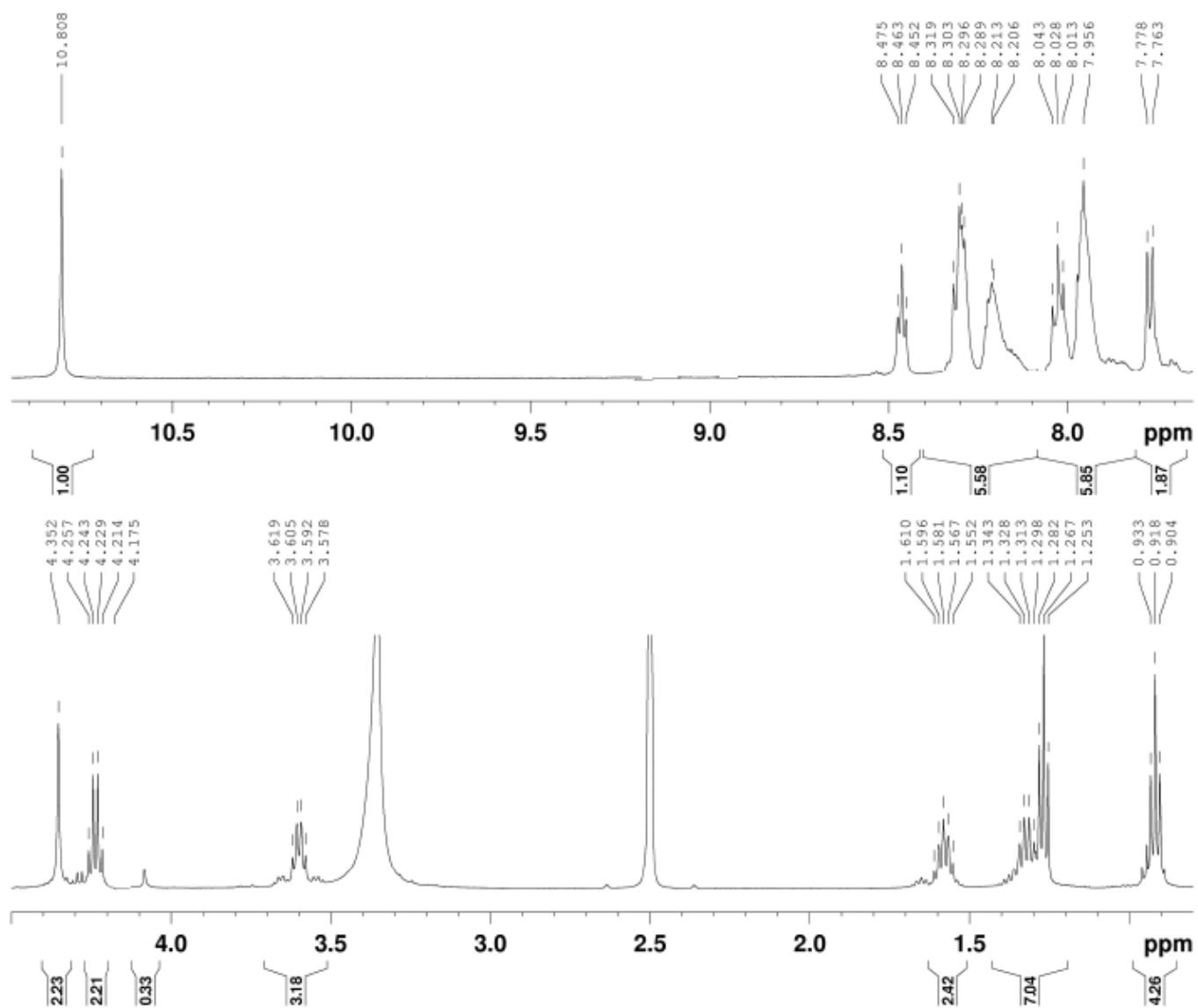
Fig. S14. Expanded ^1\text{H} NMR spectrum of 5b .
