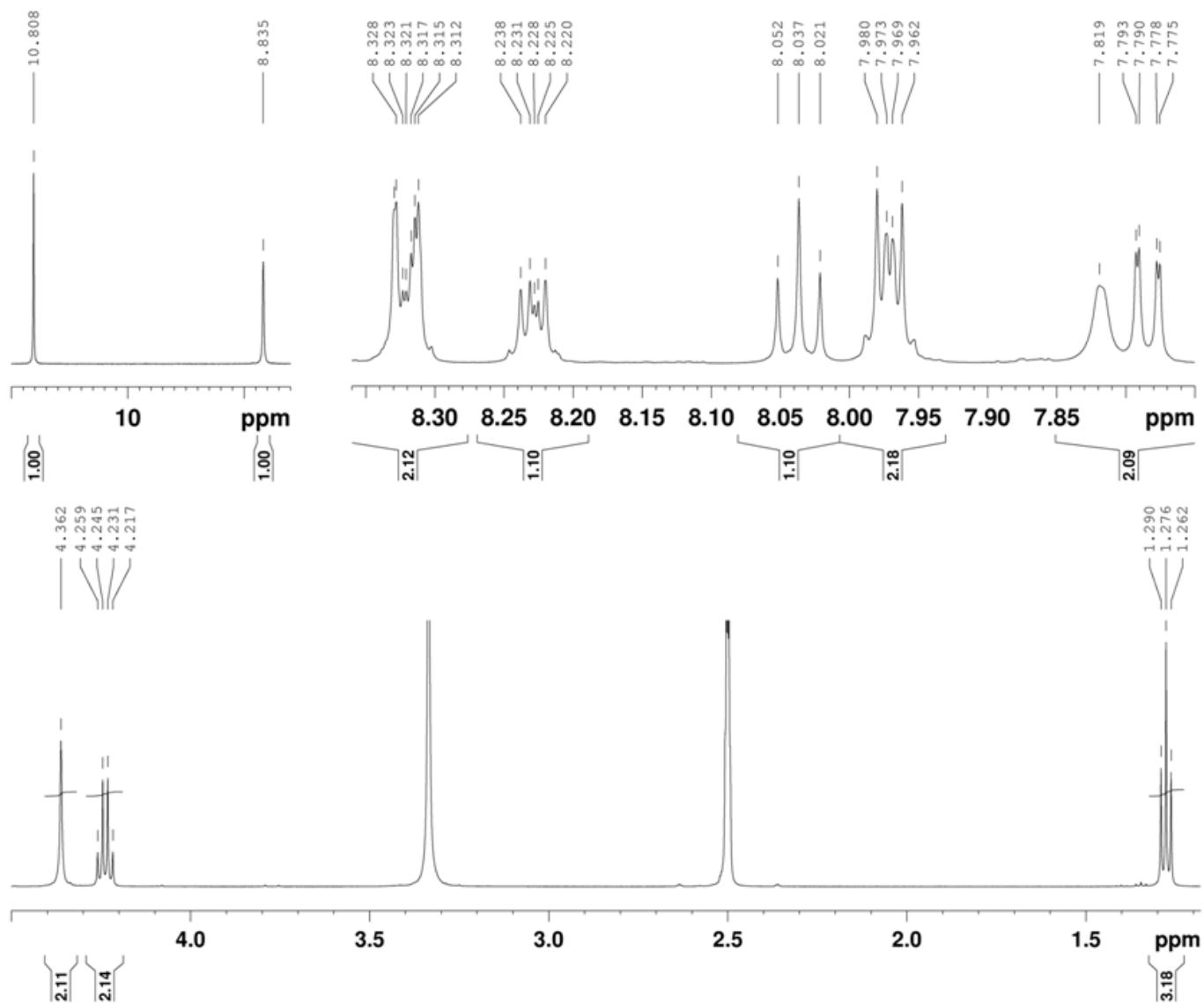
Fig. S5. Expanded 1 H NMR spectrum of 5a.
