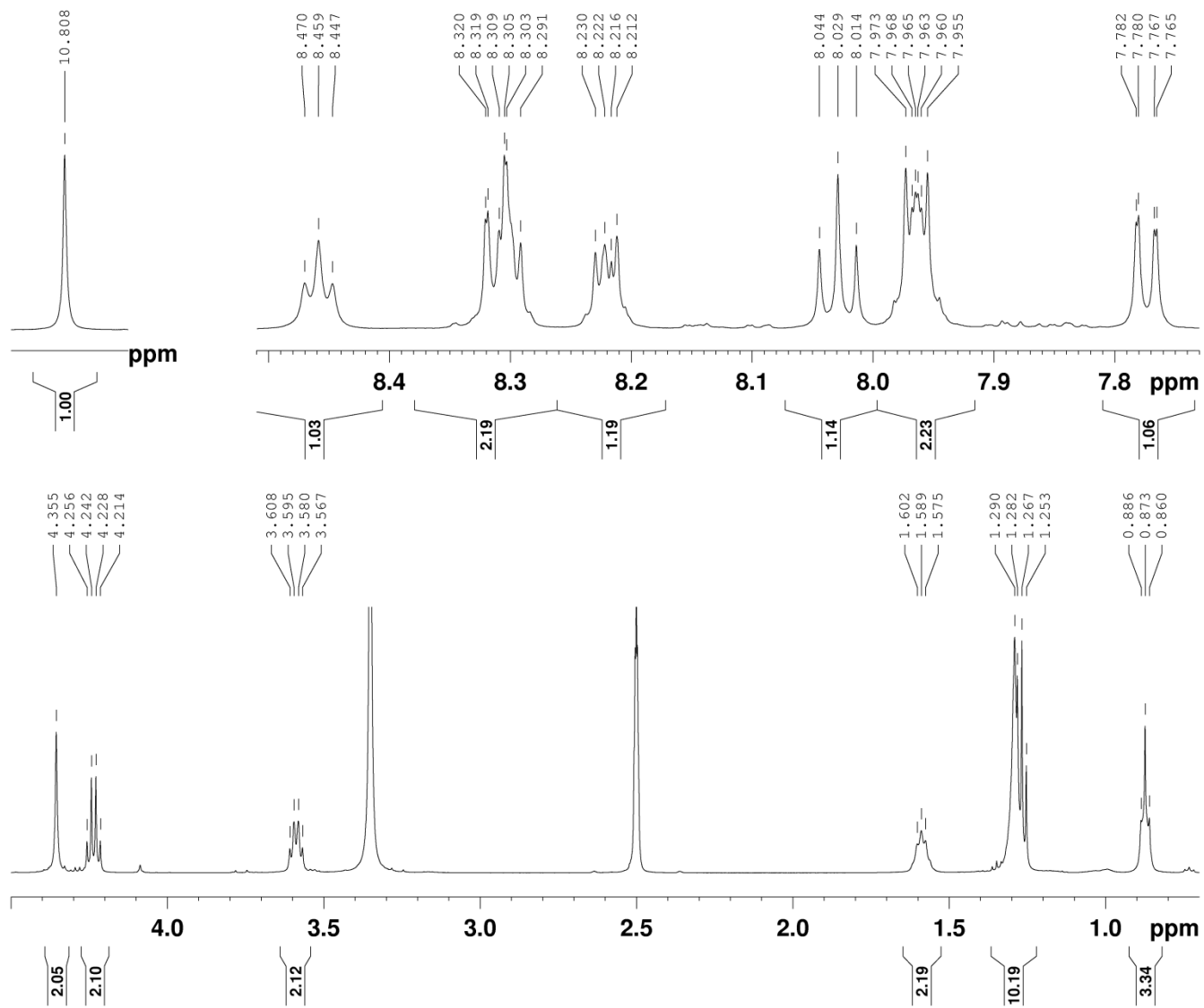
Fig. S17. Expanded ^1\text{H} NMR spectrum of 5c .
