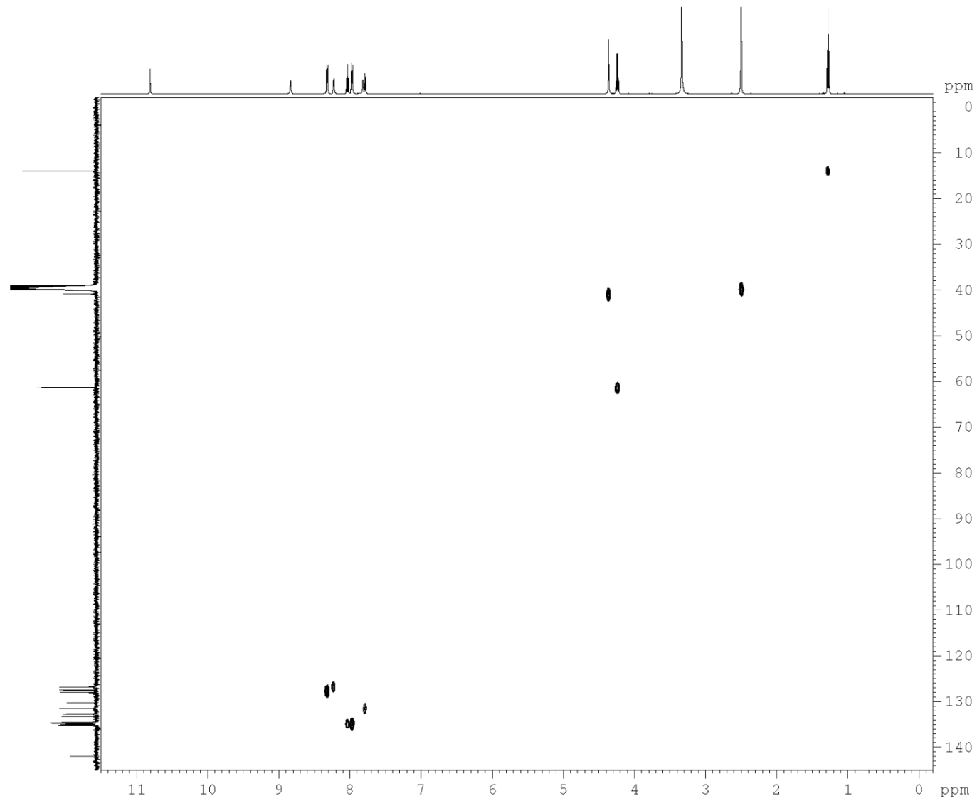
Fig. S9. HSQC spectrum of 5a .
