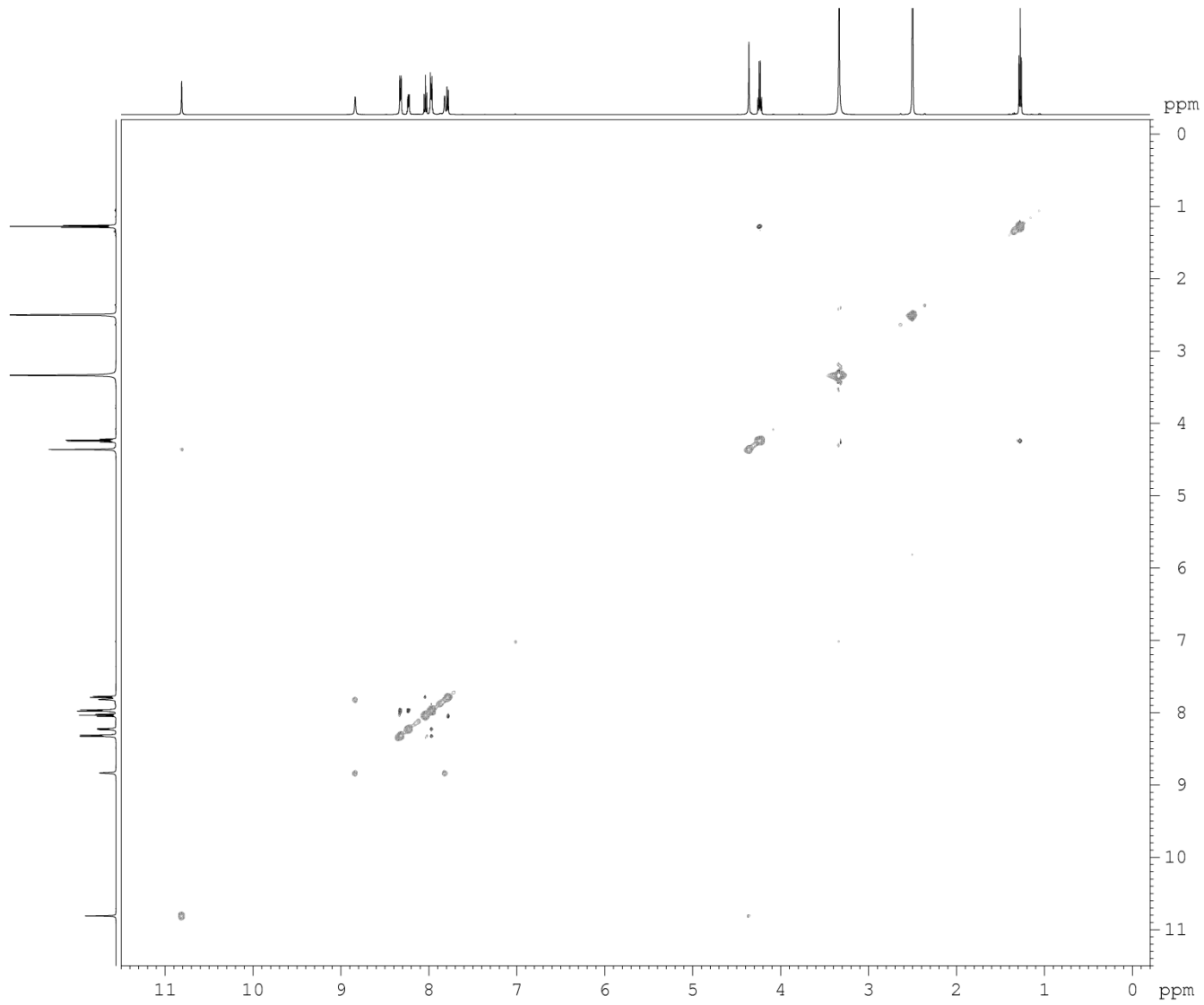
Fig. S7. NOESY spectrum of 5a .
