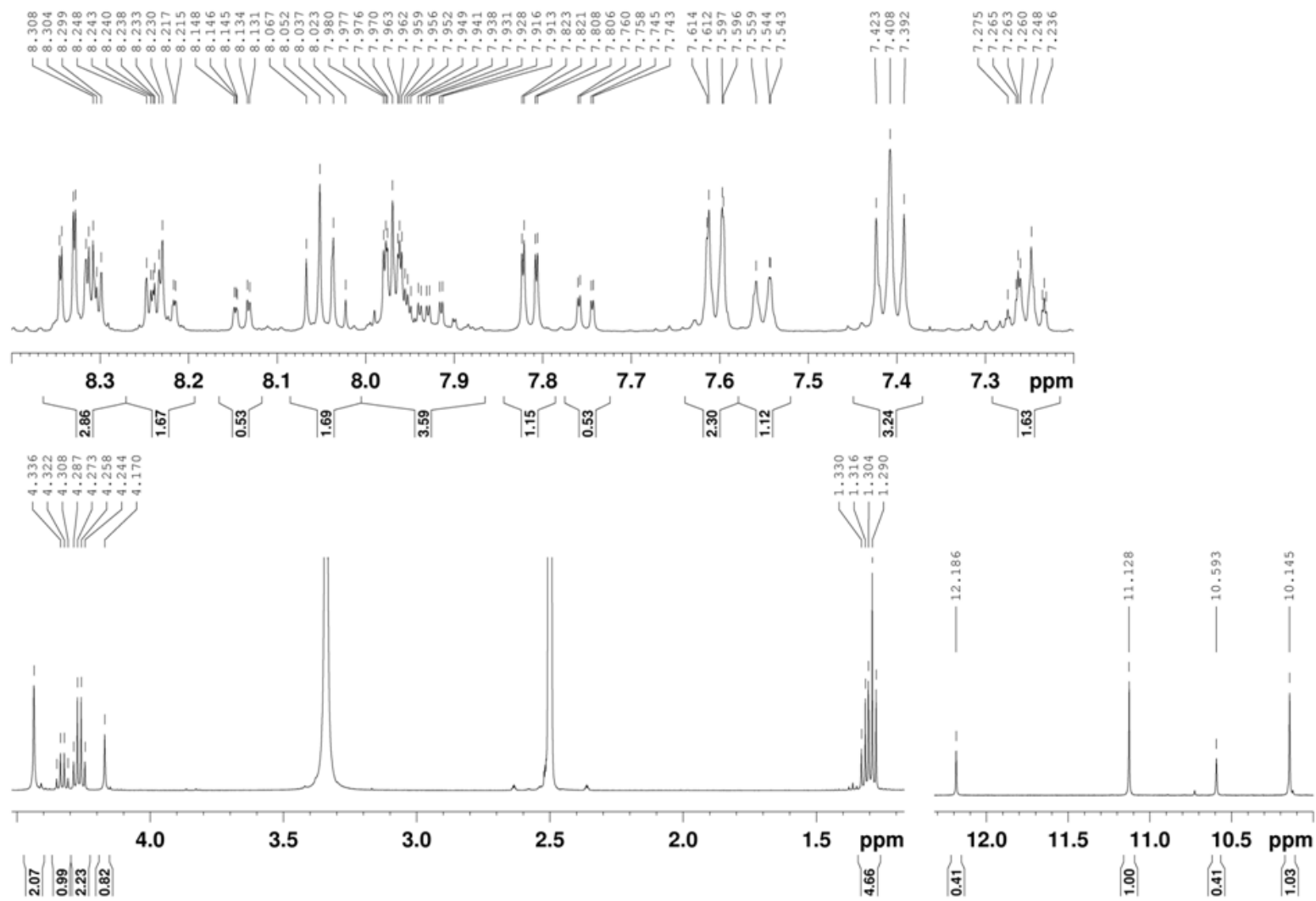
Fig. S32. Expanded ^1\text{H} NMR spectrum of 5h .
