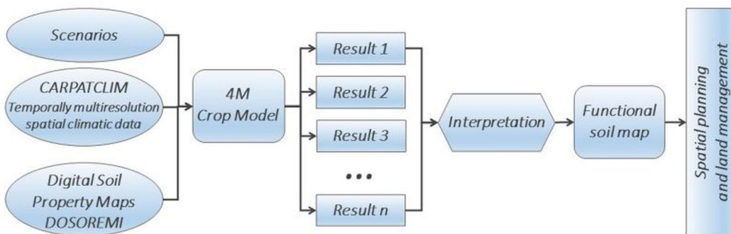
Fig. 5. Conception of mapping functional soil maps
