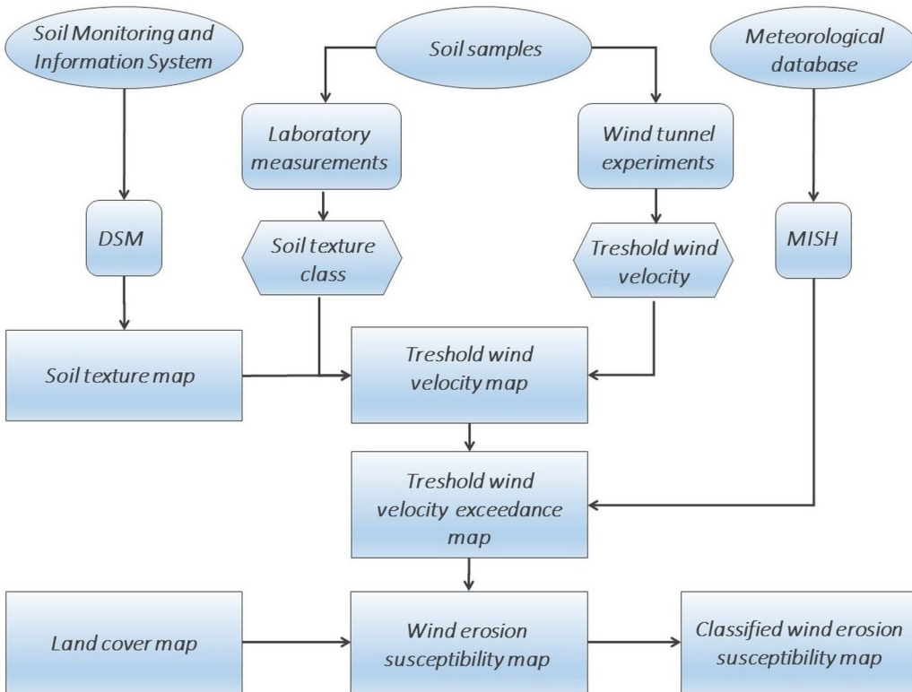
Fig. 7. Compilation process of the wind erosion susceptibility map
