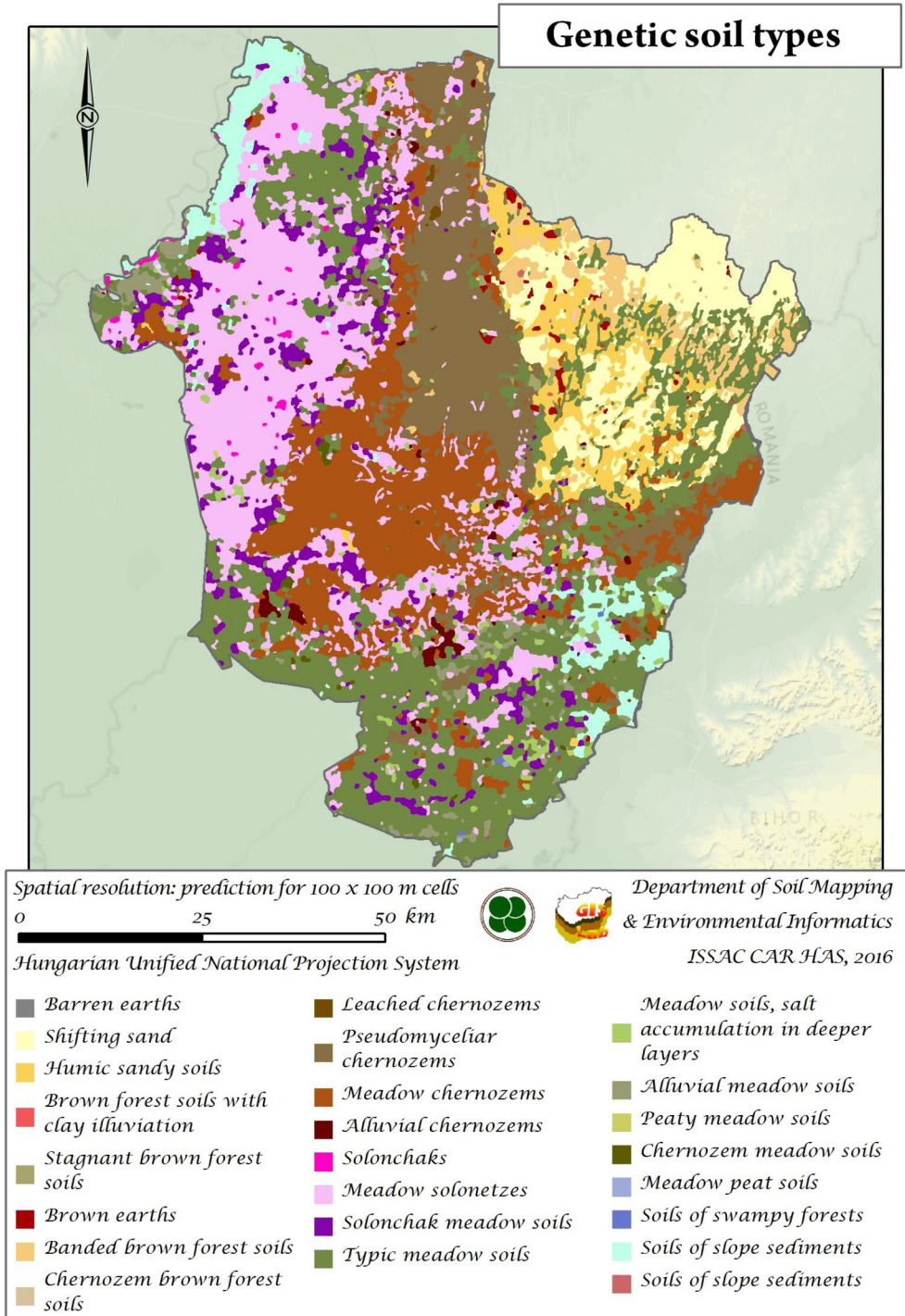
Fig. 2. Soil type map according to the Hungarian traditional genetic soil classification system
