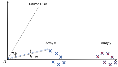
FIGURE 2. DOA estimation problem setup. Two spatially separate arrays x and y with known positions in polar coordinates, for example (l, \phi) depicted in figure above. The goal is to find \theta using n snapshots. In the diagram we have only shown one source. The effective distance with respect to the origin O is d = l \cos(\theta - \phi) .
