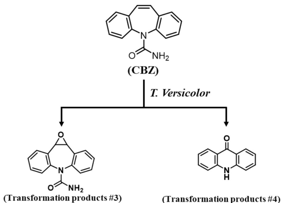
Figure 5. CBZ transformation products identified in the current study.
