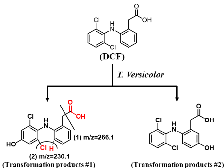
Figure 4. The two isomers of DCF transformation products identified in this study. Fragmentation of transformation product #1 is shown in red.
