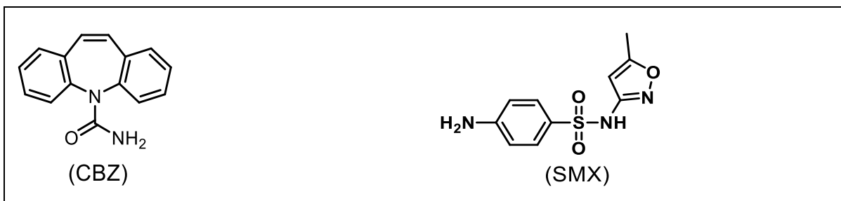
Figure 1. Chemical structures of the four PhACs selected. Diclofenac, trimethoprim, carbamazepine and sulfamethoxazole is denoted by DCF, TMP, CBZ and SMX, respectively.
