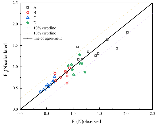
FIGURE 9. The comparison of measured results with calculated results.
