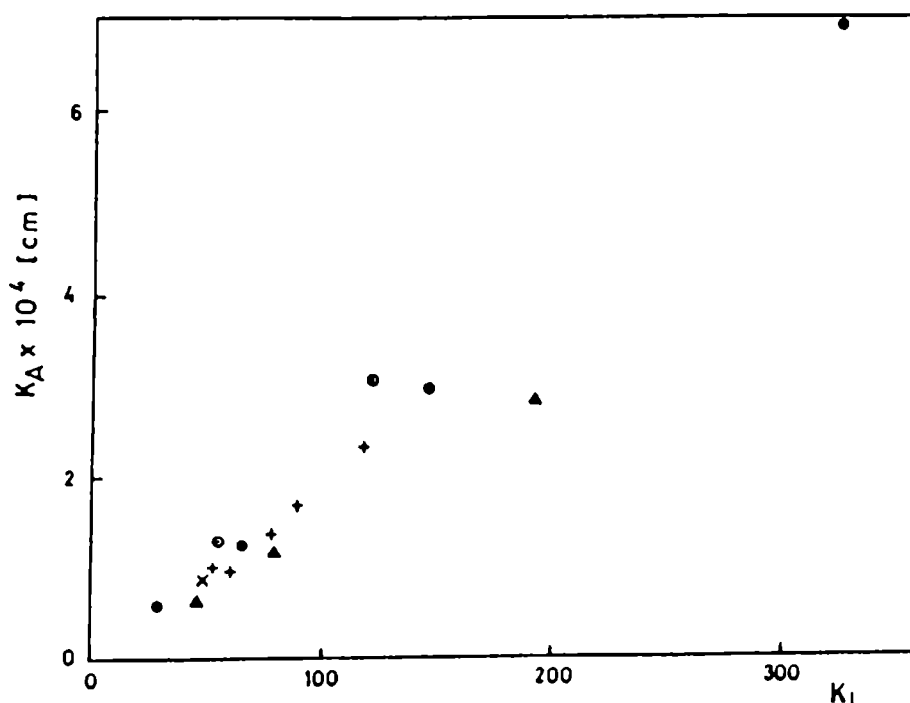
Fig. 4.- Adsorption coefficients ( K_A ) against partition coefficients ( K_L ) at 25° C. Solutes: (●) n-alkanes; (+) branched alkanes; (○) alkenes; (△) cycloalkanes; (x) cyclohexene.
