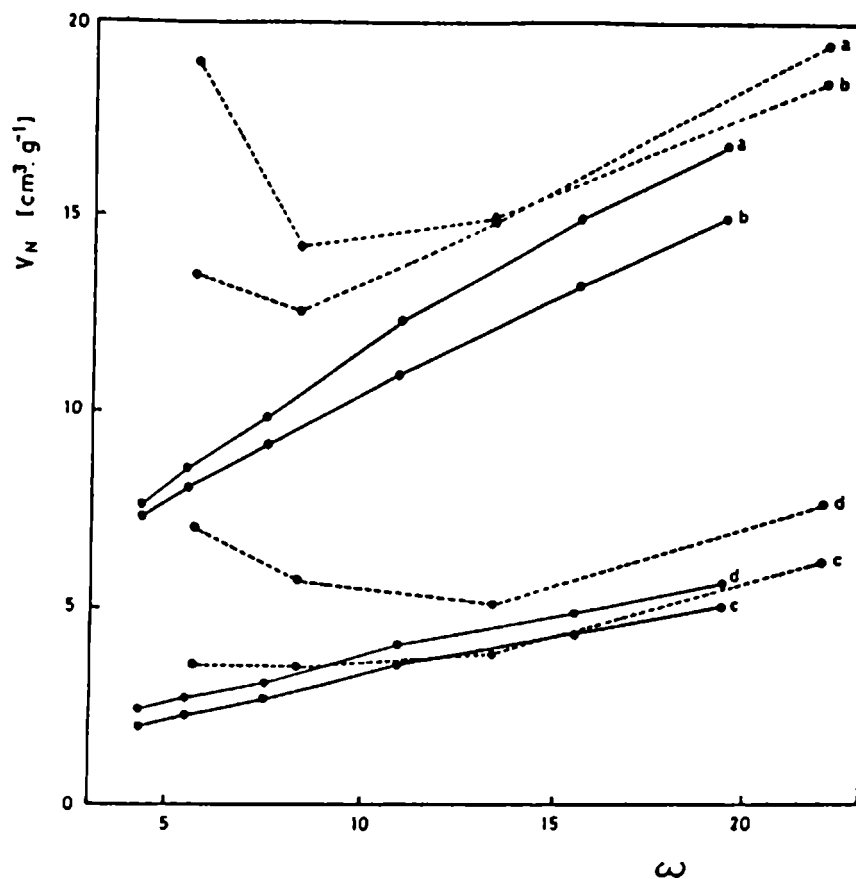
Fig. 1.- Retention volume per gram of packing at 25 °C ( V_N ) against percentage by weight of stationary phase ( w ). Dotted lines: on-column silylated packings. Continuous lines: pre-silylated packings. Solutes: (a) n-octane; (b) 1-octene; (c) cyclohexane; (d) cyclohexene.
