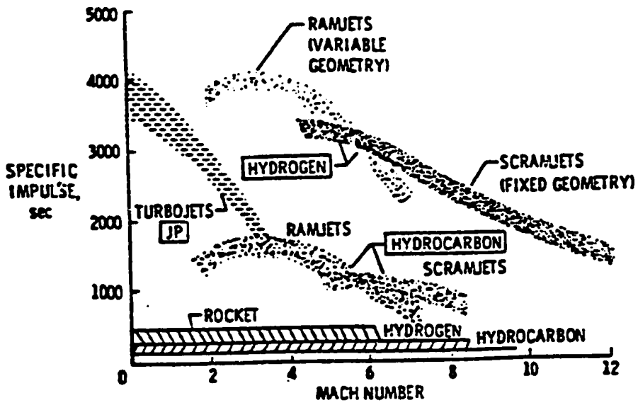
Fig. 2.1 Propulsion alternatives.
