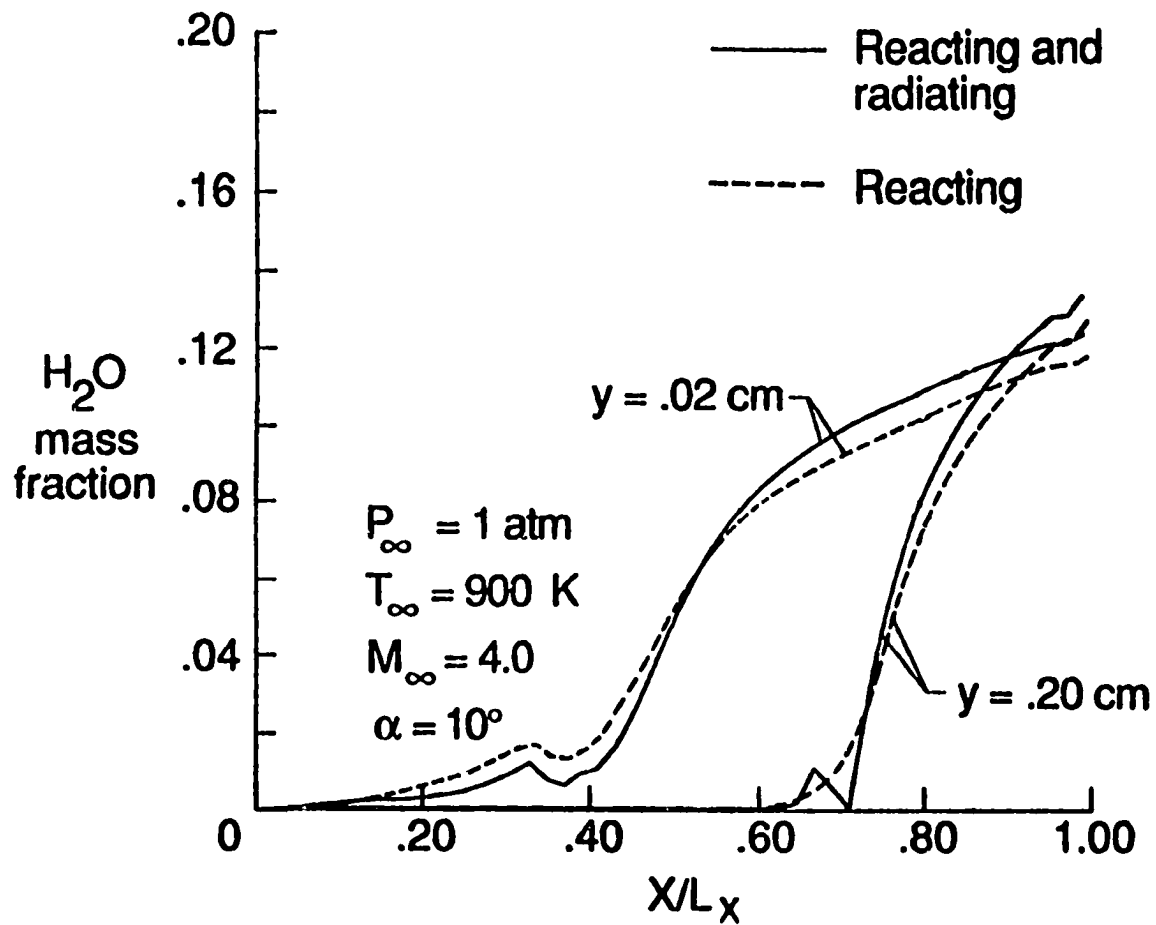
Fig. 5.55 Distribution of H_2O mass fraction along the channel for reacting and radiating, and reacting flow.
