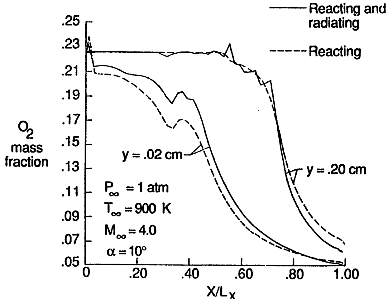
Fig. 5.56 Distribution of O_2 mass fraction along the channel for reacting and radiating, and reacting flow.
