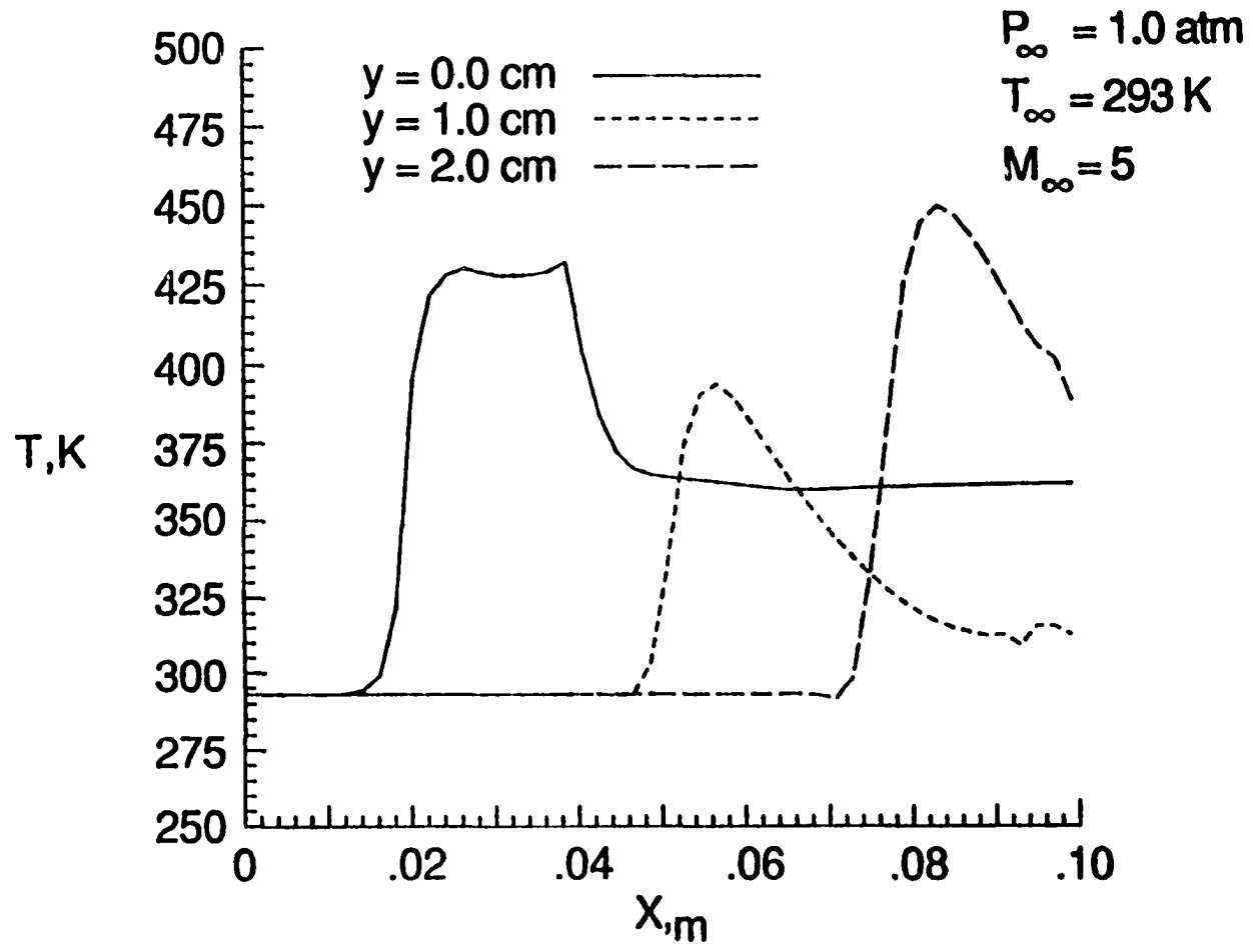
Fig. 5.5 Temperature variation with x for inviscid flow by finite volume TVD scheme.
