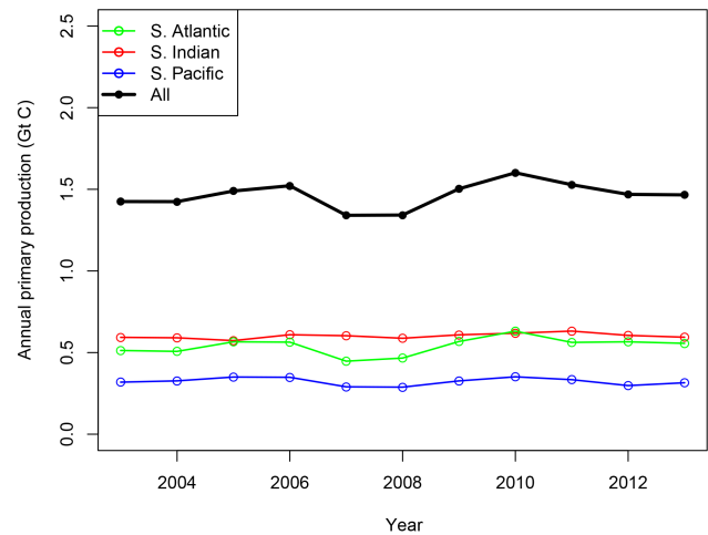
Figure 9. Temporal trend of total annual primary production by sections in the SO.
