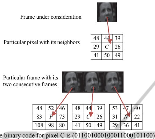
Figure 4: VDP code computation of single subject.
