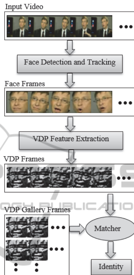
Figure 1: Video-to-video face recognition pipeline.
