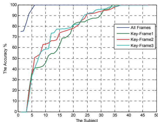
Figure 8: The accuracy for each subject for all cases.
