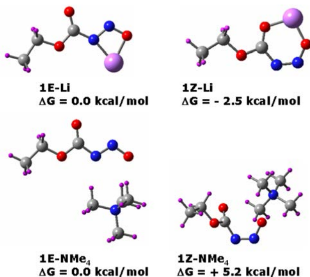
Figure 2. Optimized geometries of the Li- and Me 4 N-salts of anions 1E and 1Z . Energy differences relative to the more stable isomer in each case.
