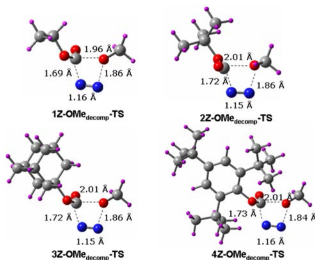
Figure 7. Optimized transition state structures for thermal decomposition of compounds ( 1Z – 4Z )-OMe.
