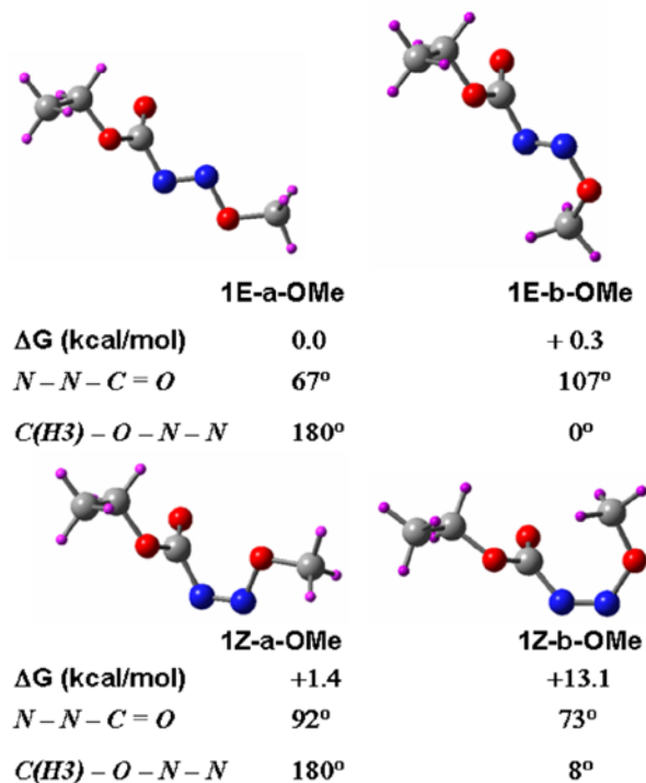
Figure 6. Optimized geometries of conformational minima of 1-OMe , with respect to the C(=O) – N, N = N and N – O bonds. Relative energies (in kcal/mol) with respect to the global minimum 1E-a-OMe .
