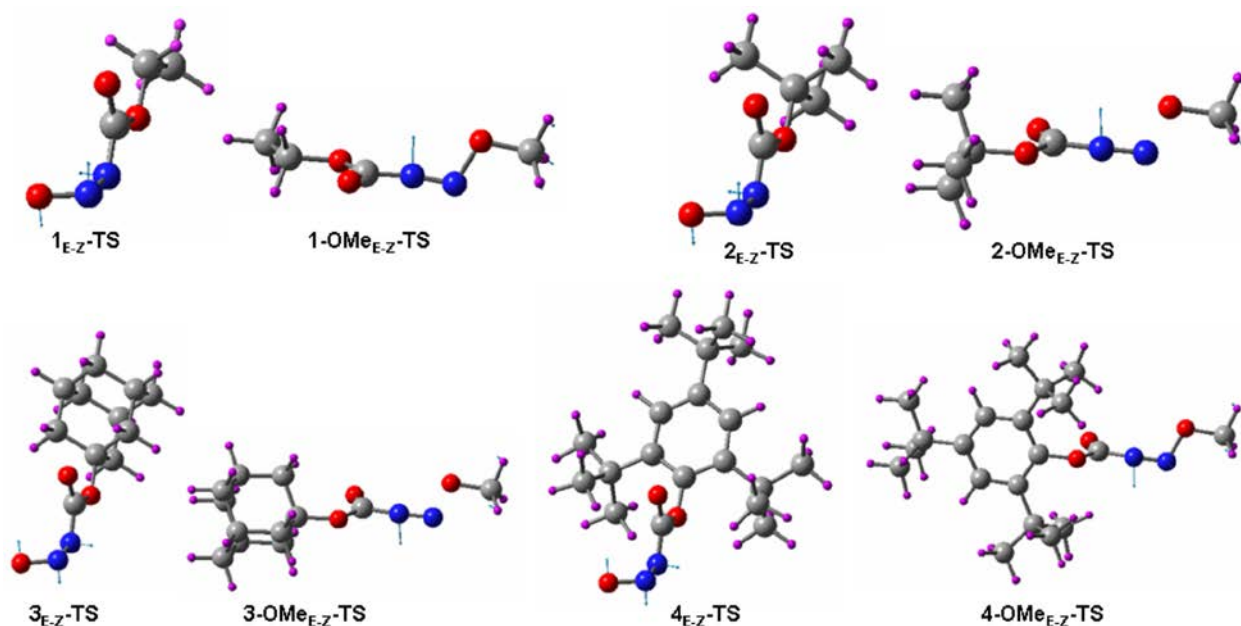
Figure 3. Optimized transition state structures for E – Z interconversion of anions 1 – 4 and their O-methylated derivatives. Displacement vectors are shown in all cases.
