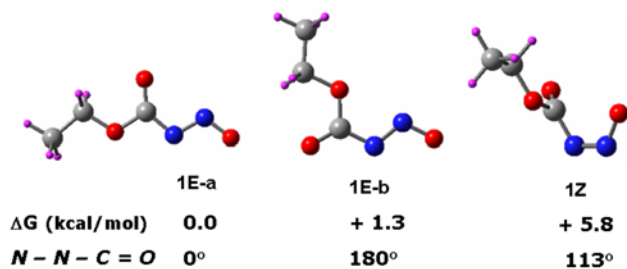
Figure 1. Optimized geometries of conformational minima of anions 1E and 1Z . Relative energies with respect to the global minimum structure 1E-a .
