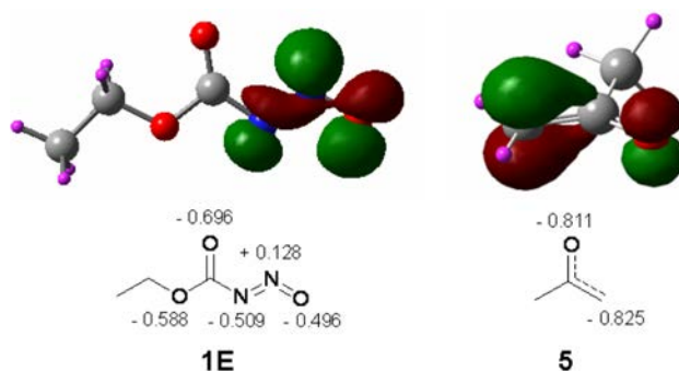
Figure 9. HOMOs and NBO charge distributions for anion 1E and acetone enolate anion 5 .
