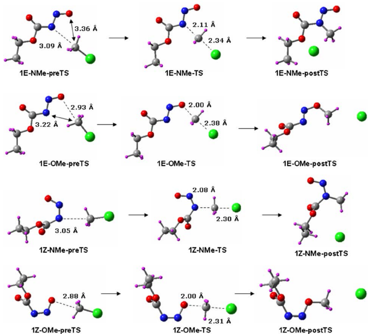
Figure 5. Stationary points for N- and O-methylation of anions 1E and 1Z . \text{CH}_3\text{Cl} was used as a methylating agent for all calculations.
