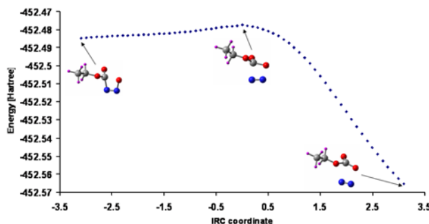
Figure 8. An IRC profile of 1Z decomp -TS, with 31 steps in each direction. Data from a B3LYP/6-31+G(d)//B3LYP/6-31+G(d) calculation
