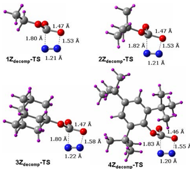
Figure 4. Optimized four-membered cyclic transition states for thermal decomposition of anions 1Z – 4Z .
