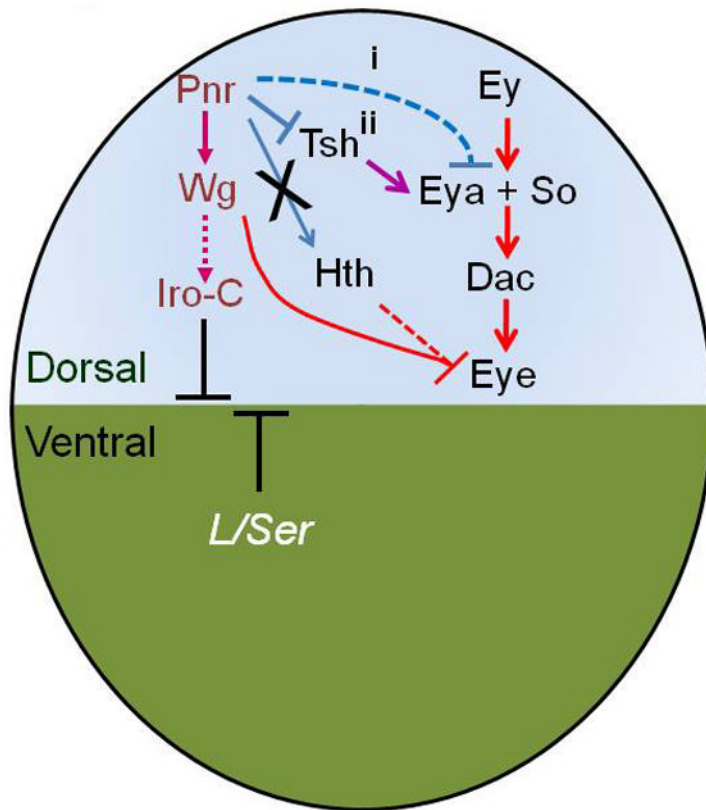
Fig. 8. Pnr suppresses the eye fate by downregulating tsh which results in suppression of retinal determination genes at the dorsal eye margin
