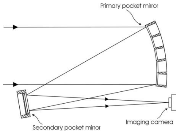
Fig.8. Telescope utilizing pocket mirrors.
