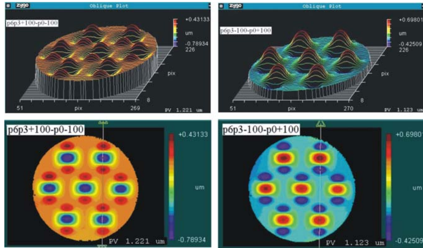
Fig.4. Left - Surface profile of 7-pocket DM if pixels (6) and (3) are at +100V, pixel (0) is at -100V. Right - opposite polarities are applied to the same pixels in each pocket.
