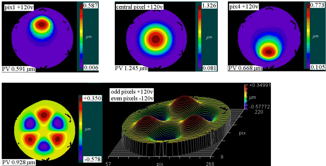
Fig.3. Response functions of one pocket when the external voltage is applied to the selected pixels.
