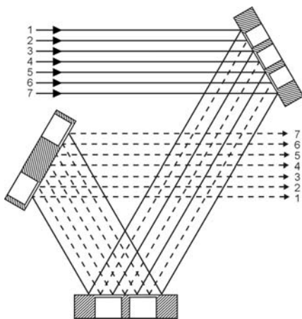
Fig.7. The part of adaptive optic system composed from pocket mirrors with overlapping control areas.
