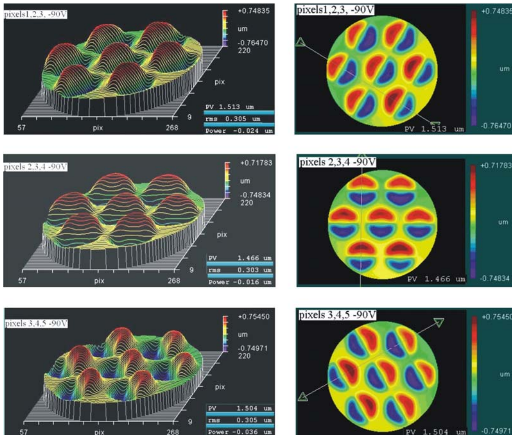
Fig.5. Surface profile of the 7-pocket mirror if three neighbor pixels are at +90V, and other three are at -90V. "Scanning" the azimuth direction.
