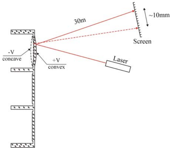
Fig.6. Setup for measurement of the resonance frequencies of the deformable areas of pockets.
