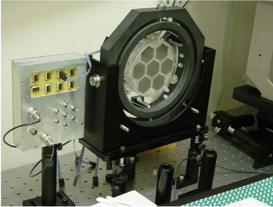
Fig.2. 7-pocket 49-channel deformable mirror with a. c. voltage station (left).
