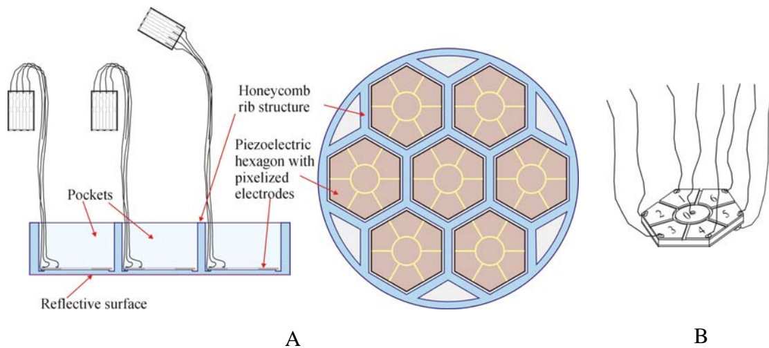
Fig. 1. A-The design of the 7-pocket deformable mirror. Each pocket contains 7 pixel piezoelectric ceramic hexagon (B), bonded to the bottom of the pocket. The electrodes on outer side of hexagon are shown by numbers from (0) to (6).
