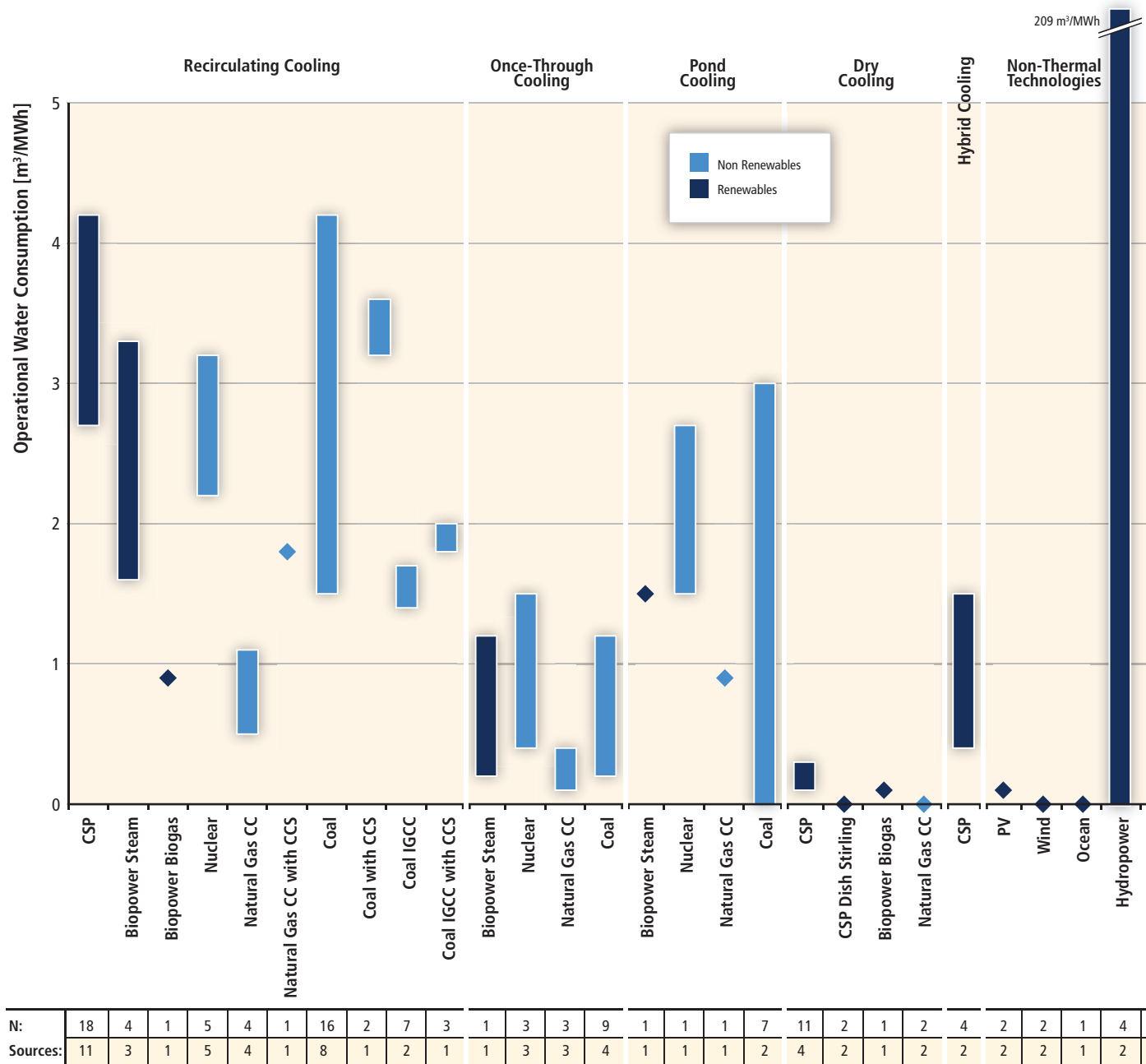
Figure 9.14 | Ranges of rates of operational water consumption by thermal and non-thermal electricity-generating technologies based on a review of available literature (m 3 /MWh). Bars represent absolute ranges from available literature, diamonds single estimates; n represents the number of estimates reported in the sources. Note that upper values for hydropower result from few studies measuring gross evaporation values, and may not be representative (see Box 5.2). Methods and references used in this literature review are reported in Annex II.
