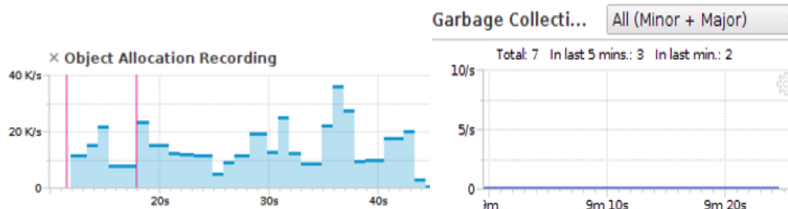
Figure 15: Object Allocation in First 40 Seconds
