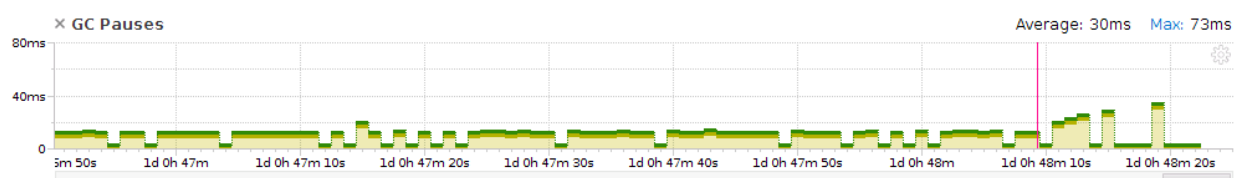
Figure 30: GC Pauses on Interaction with Web Application
