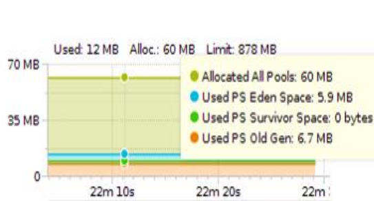
(c) Used Parallel Garbage Collector Only
