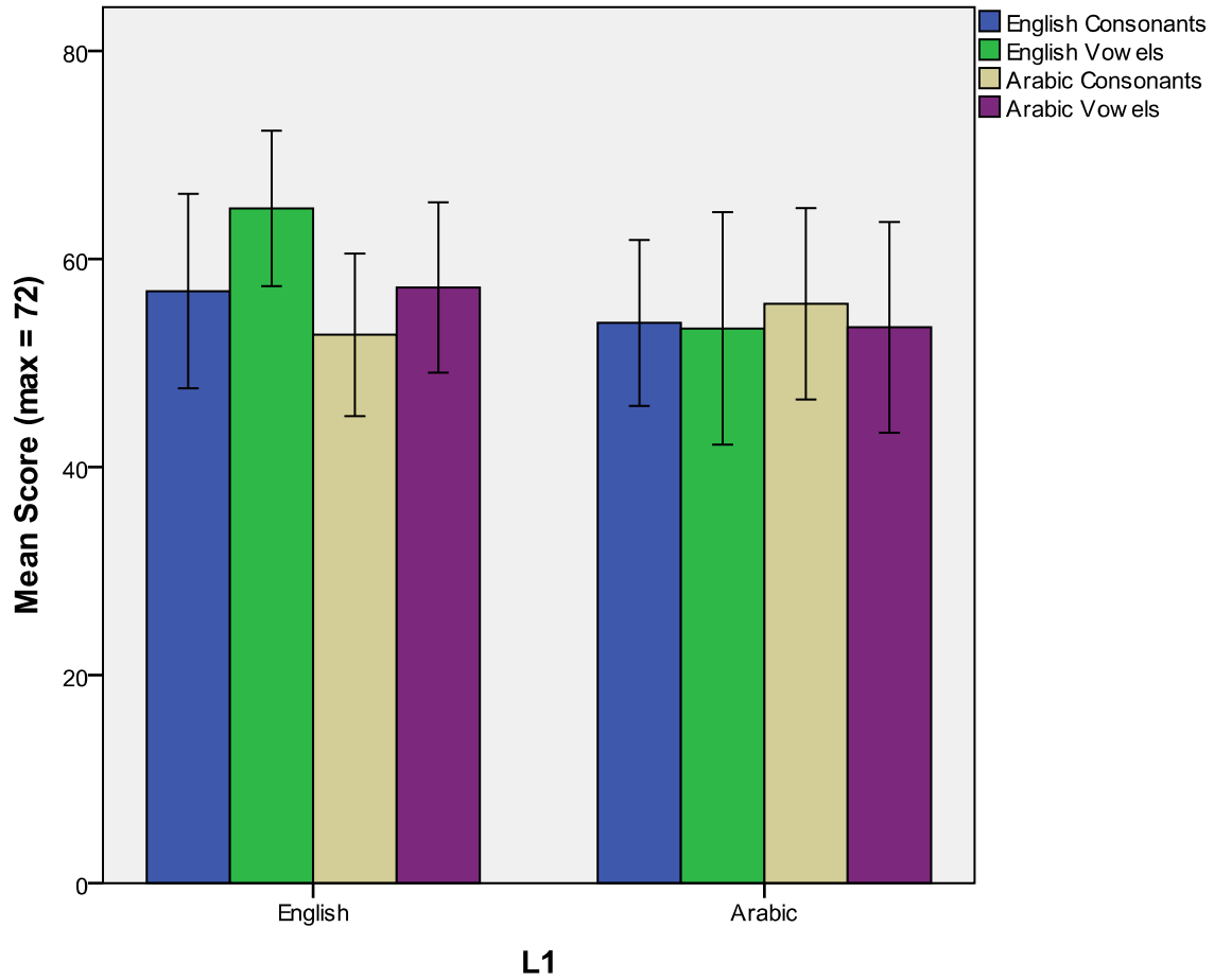
Figure 1. Mean Scores by Block and L1 Group
