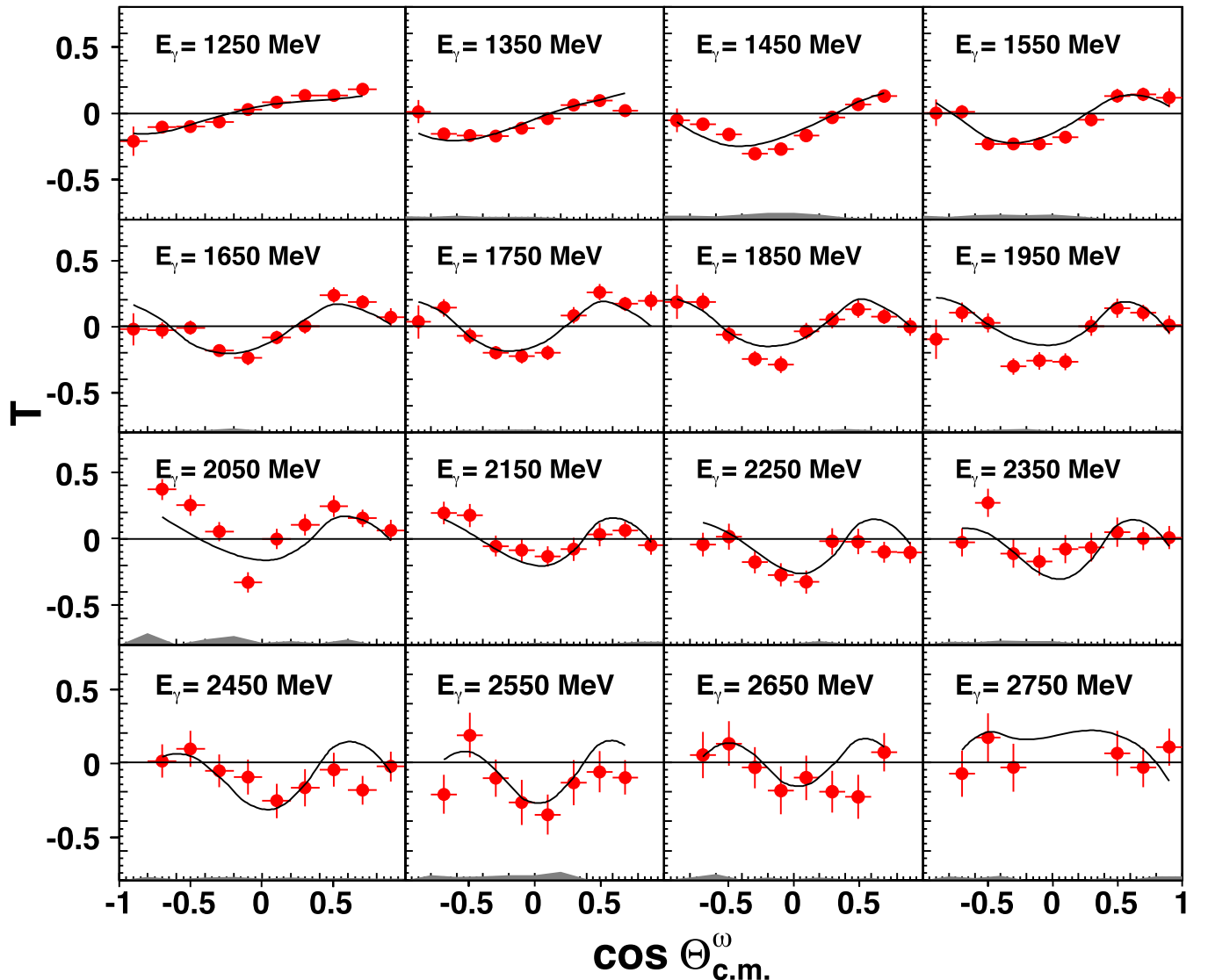
FIG. 10. Results for the target asymmetry, T , using a transversely polarized target in the reaction \gamma p \rightarrow p \omega . The data are shown for the energy range E_{\gamma} \in [1.2, 2.8] GeV in 100-MeV wide bins. The gray band at the bottom of each panel represents the absolute systematic uncertainties of our results due to the background subtraction. The horizontal bars of the FROST data points indicate the angular range they cover. The black solid line denotes the BnGa-PWA solution [40].
