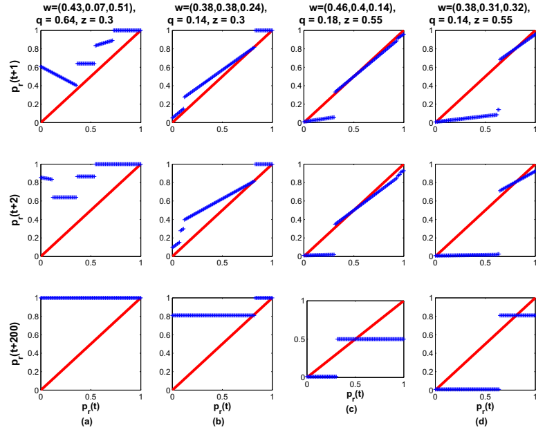
Figure 5.9: Iterations of the noisy aggregated market price (blue '+' with j = 5 versus the main diagonal (red line). Note that these parameter values yield piecewise functions with the possibility of multiple fixed points that are stable.
