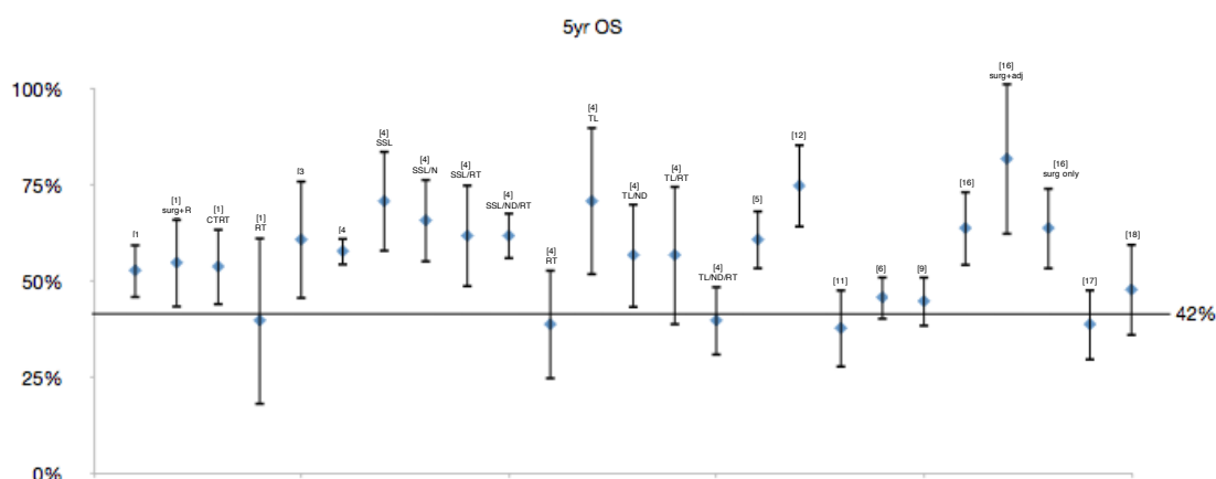
Figure 3: 5-year Overall Survival SEER-derived 5yr OS for supraglottic cancer is 42%. Individual institutional reported 5yr OS are demonstrated with hazard ratios. Bracketed numbers reference articles shown in Table 1. SSL = subtotal supraglottic laryngectomy, ND = neck dissection, RT = Radiation, TL = total laryngectomy
