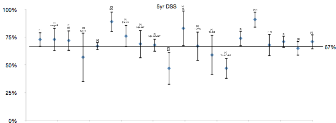
Figure 4: 5-year Disease Specific Survival SEER-derived 5yr DSS for supraglottic cancer is 67%. Individual institutional reported 5yr DS are demonstrated with hazard ratios. Bracketed numbers reference articles shown in Table 1. SSL = subtotal supraglottic laryngectomy, ND = neck dissection, RT = Radiation, TL = total laryngectomy
