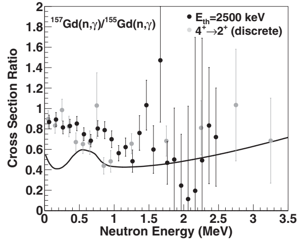
FIG. 3. The ratio of ^{157}\text{Gd}(n,\gamma)/^{155}\text{Gd}(n,\gamma) cross sections are shown for the surrogate analyses using statistical \gamma rays with E_{\text{th}} = 2.5 MeV (black points) and discrete \gamma rays using the results for 4^+ \rightarrow 2^+ transitions [20] (gray points). The smooth curve is the cross-section ratio that is calculated using reaction theory [20,25].
