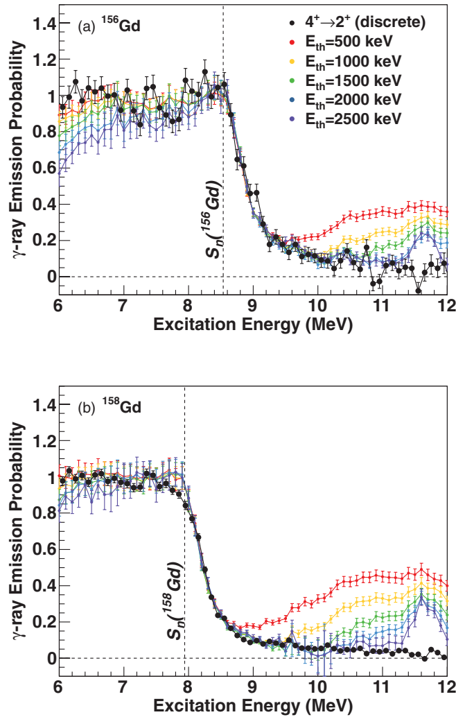
FIG. 2. (Color online) The exit-channel probability, P_{\gamma\gamma} , for (a) ^{156}\text{Gd} and (b) ^{158}\text{Gd} compound nuclei for each E_{\text{th}} value. The parameter \epsilon_\gamma is held constant at the values required to make P_{\gamma\gamma} = 1 just below S_n for each curve.
