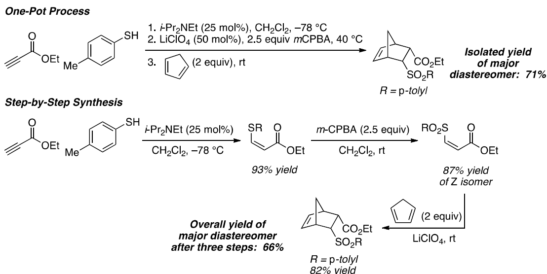
Figure 1. Comparison of one-pot reaction with step-by-step synthesis
