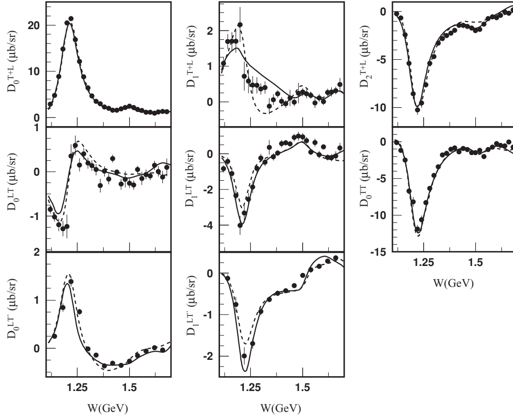
FIG. 3. Our results for the Legendre moments of the \vec{e}p \rightarrow e\pi^0 structure functions in comparison with experimental data [1] for Q^2 = 0.4 \text{ GeV}^2 . The solid (dashed) curves correspond to the results obtained using the DR (UIM) approach.
