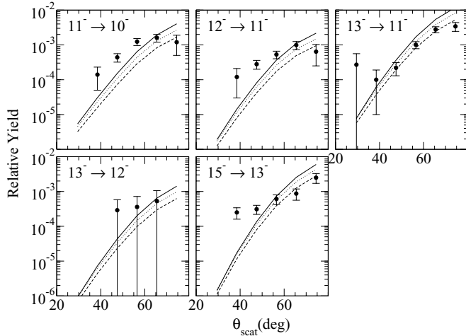
FIG. 22. Intraband yields of the 8^- isomer band and calculated yields from the best fit: total calculation (solid line), calculation for the \gamma -band \rightarrow 8^- path only (dotted line) and calculation for the GSB \rightarrow 8^- path only (dashed line).
