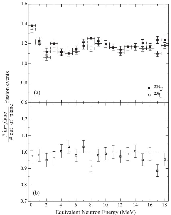
FIG. 5. Part (a) shows the ratio of in-plane versus out-of-plane fission events for ^{234}\text{U} and ^{236}\text{U} in excitation energy. Although the fission fragments were not emitted isotropically, the ratio for the two nuclei [shown in part (b)] is unity within experimental uncertainties.
