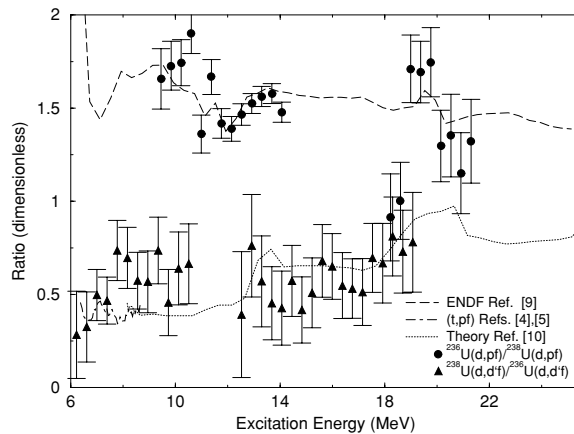
Figure 2. Fission probability ratios for the (d, pf) and (d, d'f) reactions on ^{238}\text{U} and ^{236}\text{U} targets, as a function of the excitation energy of the compound nucleus. The existing data and theoretical estimates are also indicated.
