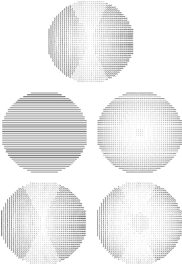
FIG. 1. Ambiguous modes of a disk. From top to bottom, m = 1, 2, 3 .
