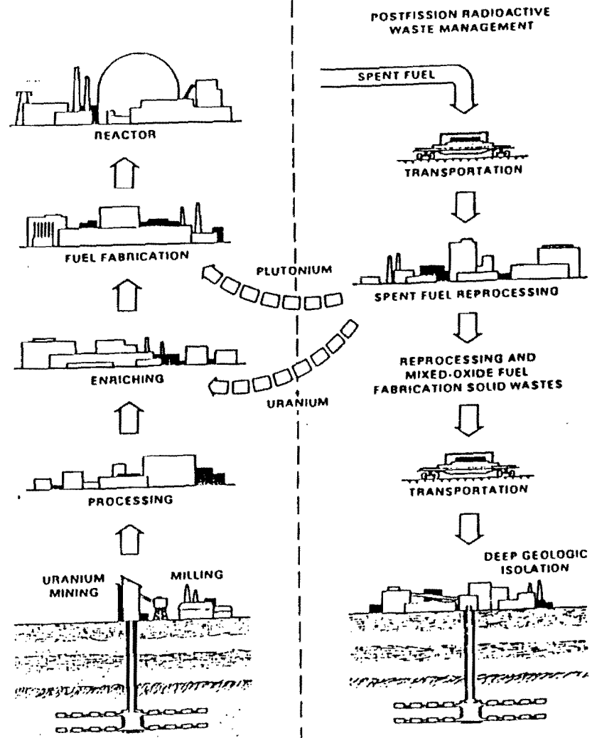
Major steps of the uranium and plutonium fuel recycle option.
