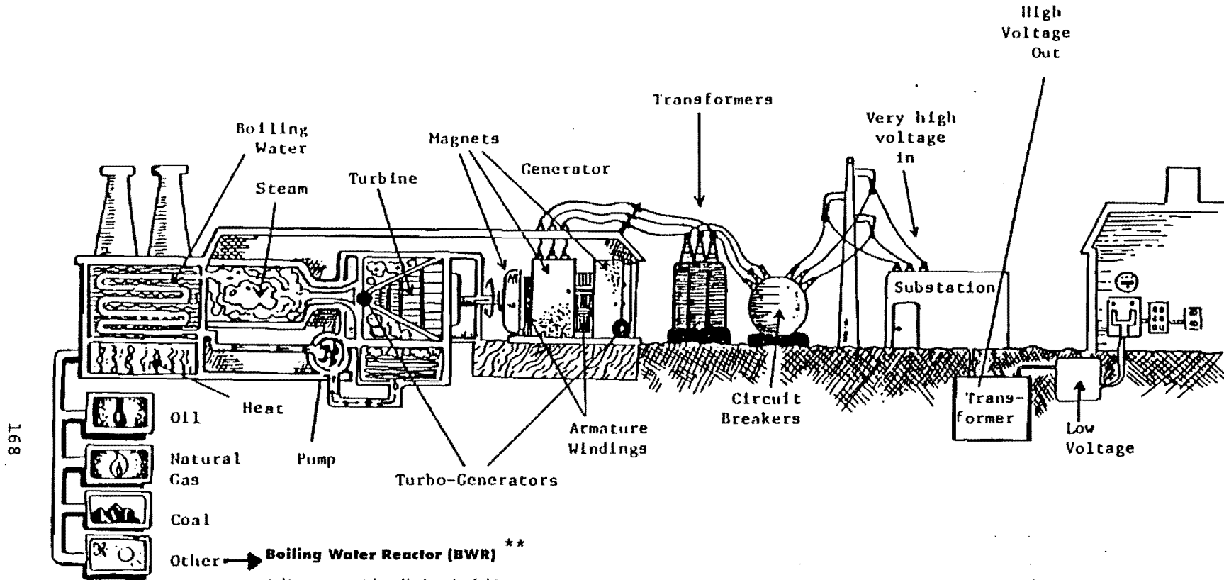
FIGURE 3 How Electricity Is Made* With nuclear power plant in inset.**
