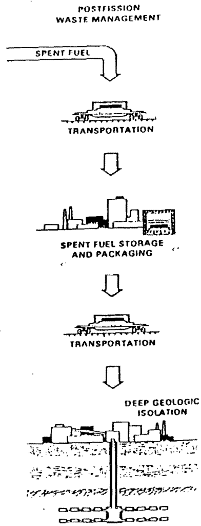
Major steps of the once-through fuel cycle option.
