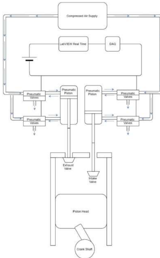
Figure 7: Initial Design of Pneumatically-Actuated Electromechanical Valvetrain
