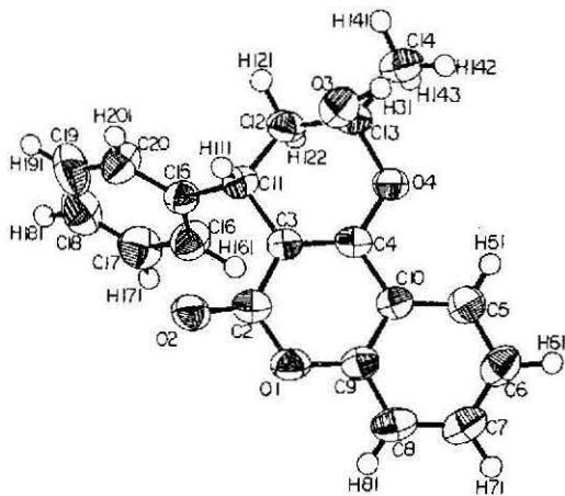
Fig. 1. Thermal-ellipsoid plot of the structure of (-)-warfarin and the numbering of the atoms. View in z direction.
