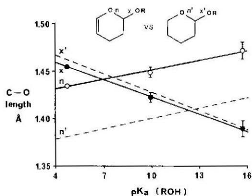
Fig. 3. A graph of C—O bond lengths in dihydropyranyl ketals from warfarin derivatives as a function of the pK a of the conjugate acid of the exocyclic ketal leaving group (solid lines). For comparison, C—O bond lengths for tetrahydropyranyl acetals are also shown (dashed lines, see text).
