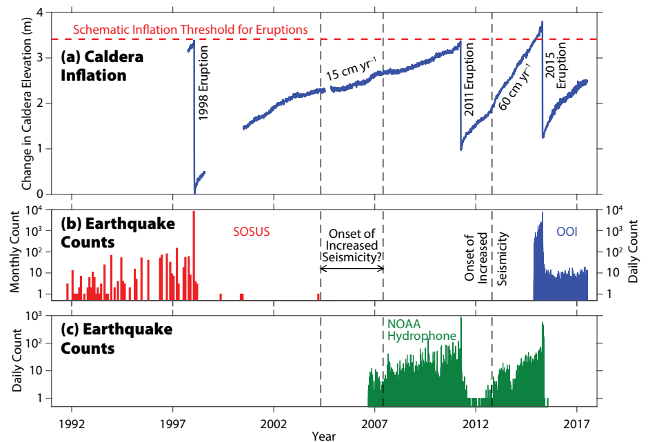
FIGURE 2. Long-term record of volcano inflation and deflation and earthquake counts at Axial Seamount. (a) Relative elevation at the center of the caldera (blue line) measured by combining data from continuously recording bottom pressure recorders with campaign-style calibration measurements from a mobile pressure recorder (modified from Nooner and Chadwick, 2016). (b–c) Histograms of earthquake counts plotted on logarithmic scales showing earthquakes detected per month by SOSUS (recreated from Dziak and Fox, 1999a), autonomous ocean bottom hydrophones (Caplan-Auerbach et al., 2017), and the OOI Cabled Array seismic network (Wilcock et al., 2016).
