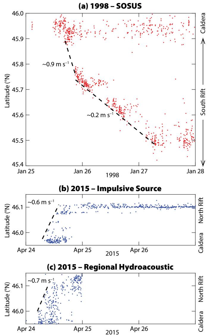
FIGURE 4. Migration of earthquakes and impulsive seafloor signals for the 1998 and 2015 eruptions. (a) Latitude of SOSUS epicenters for the first three days of the 1998 eruption (Dziak and Fox, 1999b). (b) Latitude of eruption-related seafloor impulsive signals determined with the OOI Cabled Array caldera seismic network for the 2015 eruption. (c) Latitude of earthquakes and seafloor impulsive signals for the first day of the 2015 eruption determined with hydrophones from the OOI and ONC cabled observatories (see Figure 1 inset).
