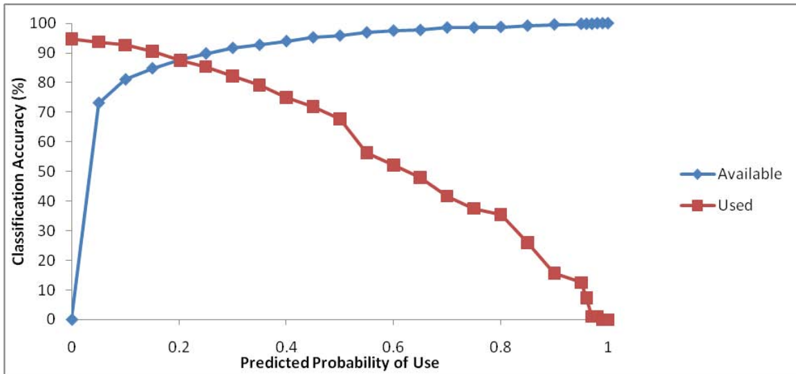
Figure 4c. Classification accuracy for used and available sites over the full range of predicted use for the composit summer model and the model-building dataset. The curves converge at a probability of 0.203 and an accuracy of 88% for both used and available paths.
