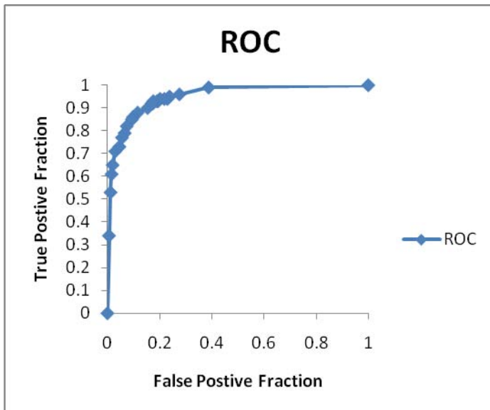
Figure 4b. ROC curve for full year data.
