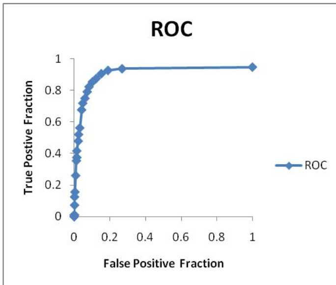
Figure 4d. ROC curve for summer data.
