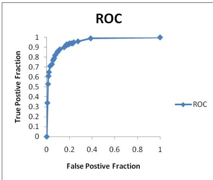
Figure 4f. ROC curve for summer data.
