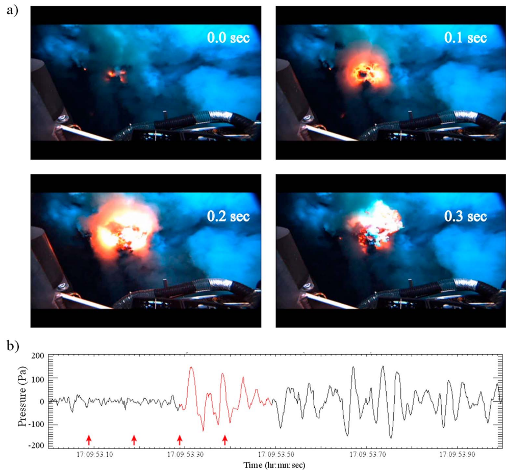
Figure 3. (a) Video image sequence of a magma gas bubble burst at West Mata Volcano summit vent Hades taken by the Jason-2 ROV [Resing et al. , 2011; Rubin et al. , 2012]. First three frames show growth of the bubble; final frame is collapse. Time shown is relative to first frame. (b) Acoustic time series of bubble growth and burst recorded by Bprobe™ hydrophone deployed 25 m from vent. Red arrows show time of the four still images in Figure 3a. No pressure signal is detected as bubble grows (frames 1–3), bubble burst causes first pressure signal peak, followed by bubble collapse (frame 4). Red part of time series shows initial bubble burst signal followed by multipath acoustic arrivals and oscillations due to response of instrument.
