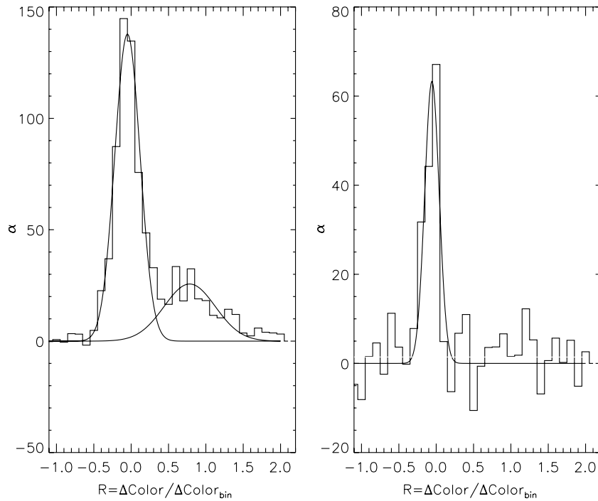
Figure 16. Relative binary fraction in the core (left) and halo (right). The single-star main sequence is centered at R = 0 , while the equal-mass binary main sequence is at R = 1 . Note the lower recovery of binary stars in the halo.
