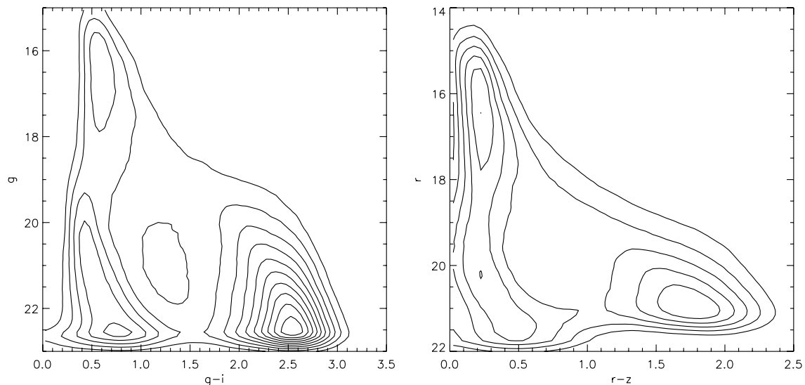
Figure 5. Smoothed background CMD filters, n_{\text{bg}}(g-i, g) (left), and n_{\text{bg}}(r-z, r) (right). The sample is drawn from a region around M67 with 1^\circ < \text{radius} < 8^\circ . The contours are in increments of \frac{1}{2}\sigma above the mean. Specific features are discussed in the text.
