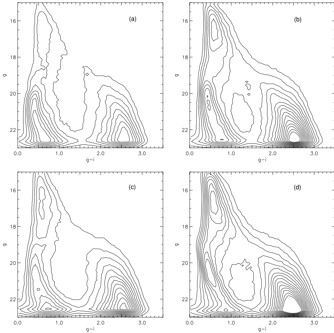
Figure 4. Background filters n_{\text{bg}}(g-i, g) of four 5^\circ \times 5^\circ regions in our sample. The (R.A., decl.) centers of each region are (a) (138.5,17.5), (b) (127.5,17.5), (c) (138.5,5.5), and (d) (127.5,5.5). Region (d) greatly overlaps the missing data seen in Figure 1, but the qualitative features seen in panel (d) above are sufficient for our needs. Contours in all four panels are in steps of \frac{1}{2}\sigma_a above the mean level of panel (a) to demonstrate the increasing stellar density at lower galactic latitudes. Specific features are discussed in the text.
