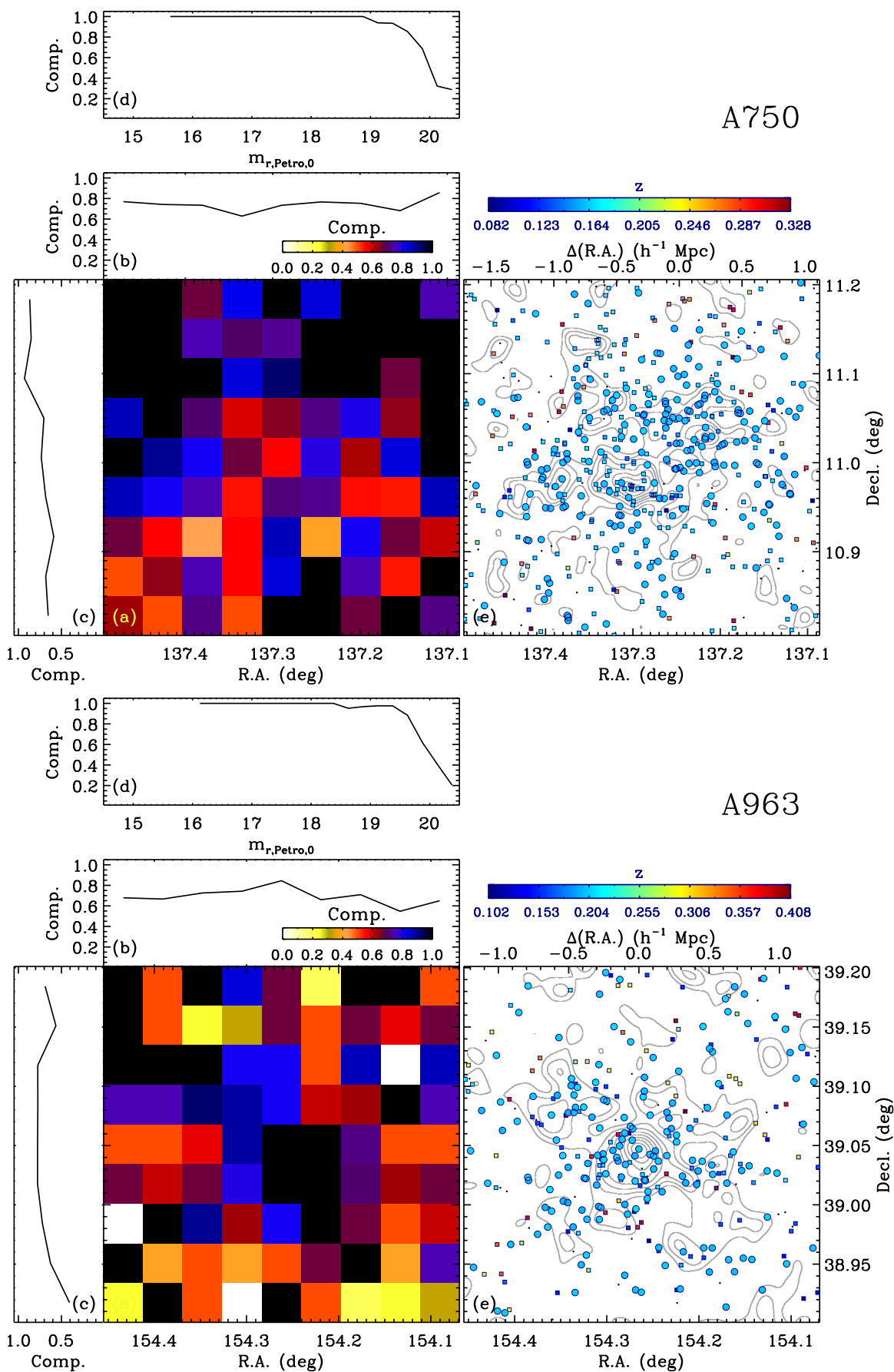
Figure 16. Same as Figure 4, but for A750 and A963.
