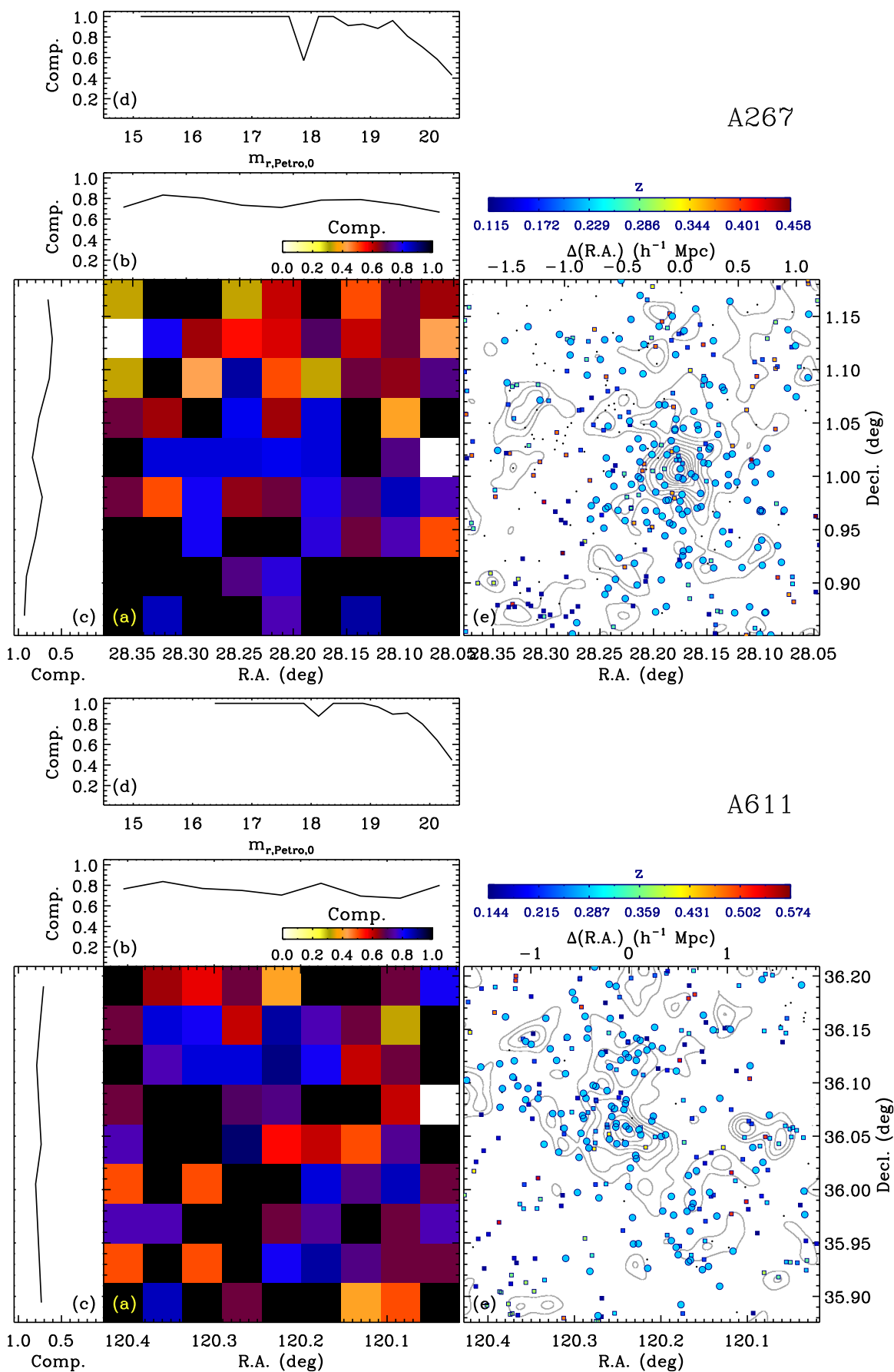
Figure 14. Same as Figure 4, but for A267 and A611. (A color version of this figure is available in the online journal.)
