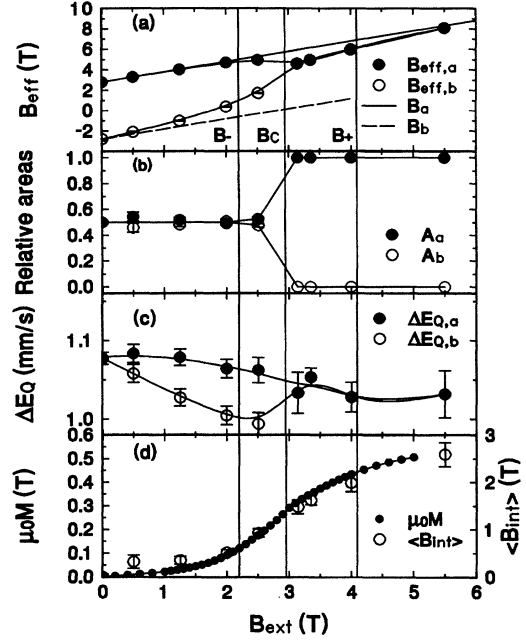
FIG. 13. Results for the spectra for T=10.1 K, parallel field. (a) The effective hyperfine fields B_{\text{eff},a} and B_{\text{eff},b} ; the lines B_a = B_{\text{eff},a}(10.1 K, 0 T) + B_{\text{ext}} and B_b = B_{\text{eff},b}(10.1 K, 0 T) + B_{\text{ext}} are shown. The lower field B_- and upper field B_+ denoting the maxima in the imaginary component of the ac susceptibility from Ref. 7 as discussed in the text are shown as well. (b) The areas A_a and A_b . (c) The EFG \Delta E_{Q,a} and \Delta E_{Q,b} are shown. (d) The bulk \mu_0 M from Ref. 7 is compared with the local magnetization B_{\text{eff},a}A_a + B_{\text{eff},b}A_b . Lines are guides for the eye.
