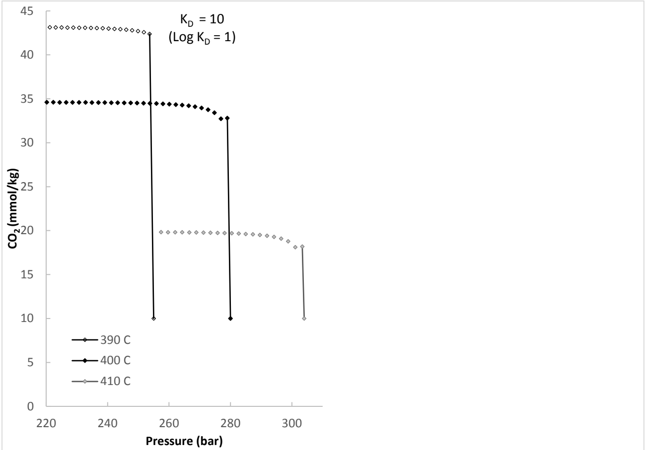
Figure S1. Simple model demonstrating the relative influence of K_D , and temperature on the extent of volatile enrichment upon initial phase separation (reflected by the jump in \text{CO}_2 concentration at depth) and the insensitivity of volatile concentrations to subsequent supercritical phase separation (reflected by nearly horizontal lines of \text{CO}_2 vs. pressure). In this illustration, as vapor phase fluid rises, at every stage the vapor is segregated, and moves upward. No remixing with the brine is allowed and no temperature change takes place.
