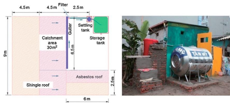
Figure 6 – Rainwater harvesting tank in Hanoi [10]
