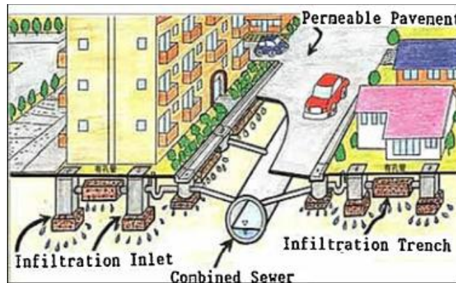
Figure 5 – Tokyo’s Infiltration System [10]
