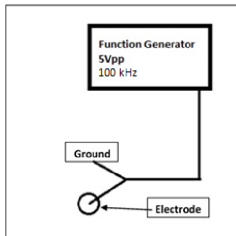
Figure 8: Alpha Prototype setup.
