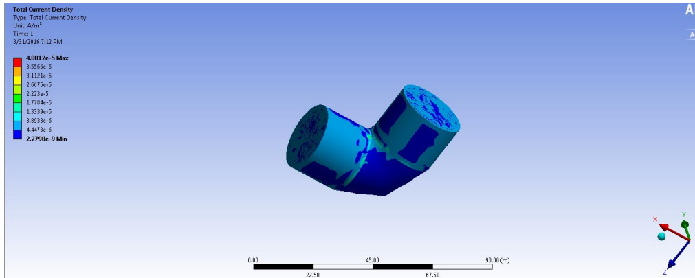
Figure 5: Leg-joint model stimulated by 10V at joint. Multiple layers of materials are present and able to be customized to fit the isotropic resistivities of human tissue.
