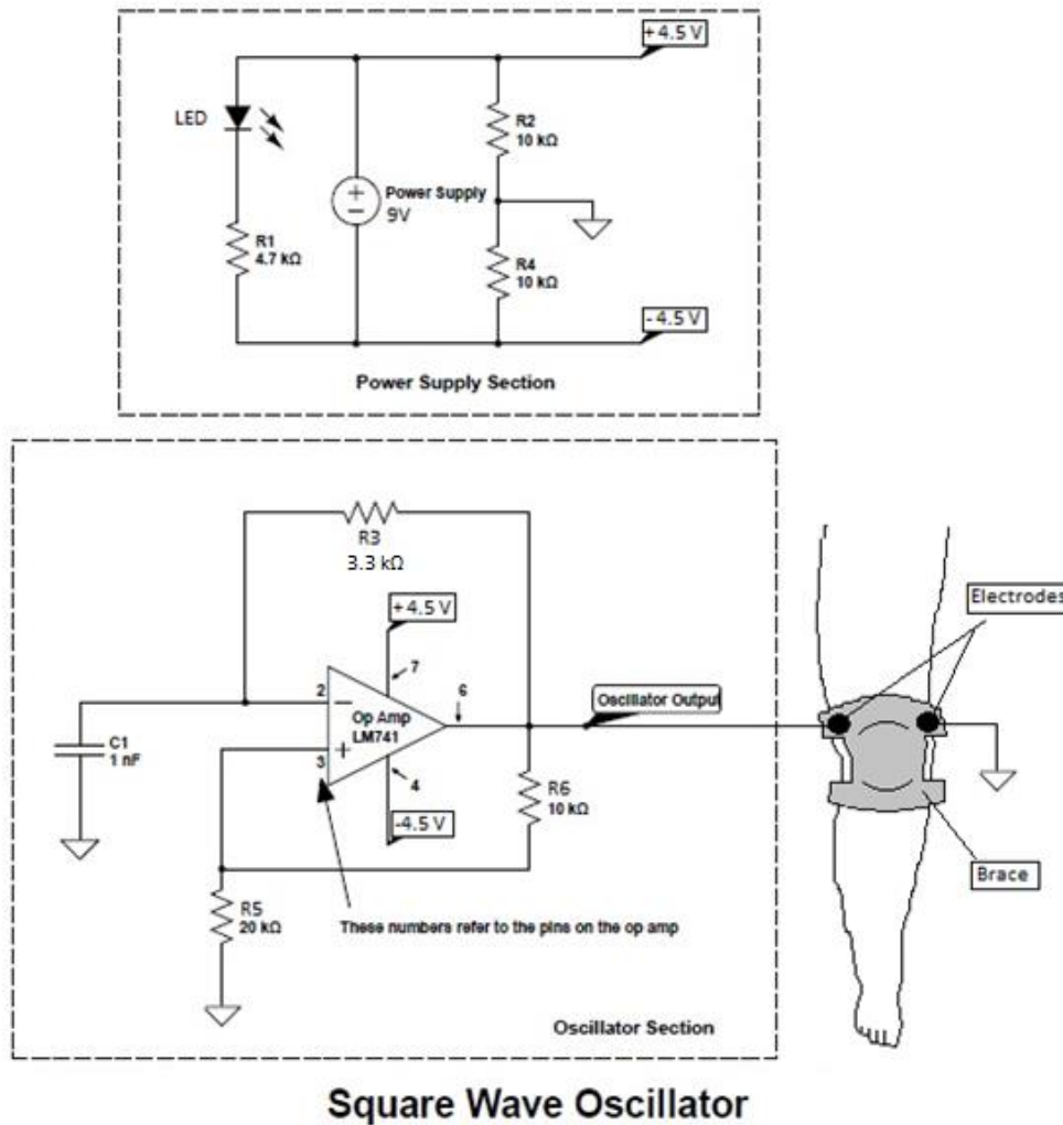
Figure 10: Square wave oscillator circuit schematic and sketch of the brace with electrodes on a leg.
