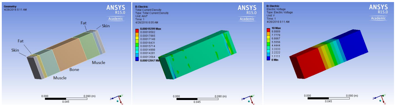
Figure 6: Left image shows geometry of scalable model. The center image shows the current distribution using two points of contact on the left and right end of the geometry. The right image shows the voltage drop with the same set-up.
