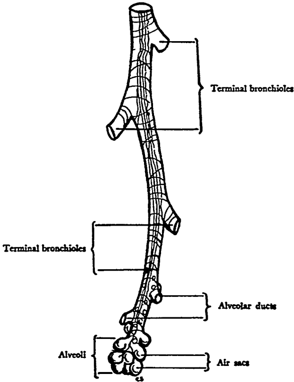
Fig. 2. Architecture Structural units of the lung tissue.
