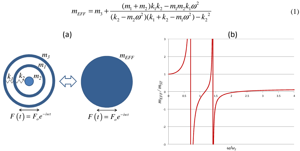
Fig. 1: (a) Dual-resonator spring-mass system and its effective mass model, (b) Plot of m_{EFF}/m_{ST} against \omega/\omega_2 .
