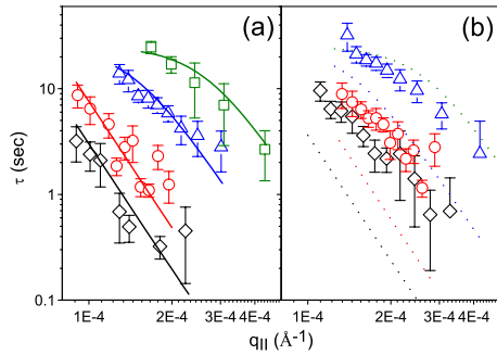
FIG. 4 (color online). The values of \tau as a function of q_{||} for 220 ( \square ), 490 ( \triangle ), 660 ( \circ ), and 900 ( \diamond ) Å thick C18 films at 331.2 K (a) and 327.2 K (b). The data for 220 Å thick film are not plotted at 327.2 K as time independent g_2 was observed (see text). The solid lines in (a) are the fits using the viscous model for 660 and 900 Å thick film and using viscoelastic model for 220 and 490 Å thick film (viscosity of 125 Pa s and shear modulus of 5 Pa). Shown as dotted lines in (b) are the calculated values of \tau using the viscous model for 660 and 900 Å thick films and using a viscoelastic model for 220 and 490 Å thick films. We have taken into account the small differences in the bulk viscosity (3.6 Pa s) and surface tension ( -0.7 mN/m [9]) between 331.2 K (above T_s ) and 327.2 K (below T_s ).
