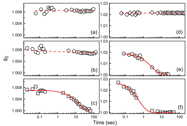
FIG. 3 (color online). Autocorrelation function ( g_2 ) obtained for C18 at q_{\parallel} = 1.65 \times 10^{-4} \text{ \AA}^{-1} measured on 220 Å (a)–(c) and 660 Å (d)–(f) thick films. The data are shown for T < T_m (316.2 K) [(a),(d)], T_m < T < T_s (327.2 K) [(b),(e)], and T > T_s (331.2 K) [(c),(f)]. The solid lines are the single-exponential fits to the data to obtain the relaxation time \tau . The dashed lines are the linear guides for the eye.
