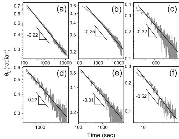
FIG. 2. \theta_t during the late-stage meniscus relaxation process as a function of time in a log-log plot. The values are calculated using the force data as described in the text. The data are plotted for relaxation with a Pt wire of C18 at 328.0 K (a), C22 at 342.7 K (b), C18–C22 blend with 2 wt. % bulk concentration of C22 at 339.7 K (c). We have also plotted the relaxation of C18 at 328.0 K in contact with a glass wire (d), and a PS-coated Pt wire (e). The relaxation of PDMS with a Pt wire at 298.0 K is shown in (f). The solid lines are the power-law fits (the error of the fits were \pm 0.01 ) to the data.
