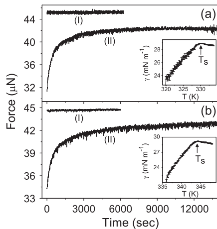
FIG. 1. The force experienced by the Pt wire during meniscus relaxation as a function of time for C18 (a) and C22 (b). The data are shown for T > T_s (C18, 330.1 K; C22, 344.2 K) (I), and T_m < T < T_s (C18, 328.0 K; C22, 342.7 K) (II). The insets represent the static \gamma of C18 (a) and C22 (b) measured in the heating cycles [9]. The arrows indicate T_s for the respective polymers. The meniscus relaxes within the experimental time resolution of 1 sec at T > T_s . In contrast, it relaxes over a period of 4–6 hr upon decreasing the temperature to T < T_s .
