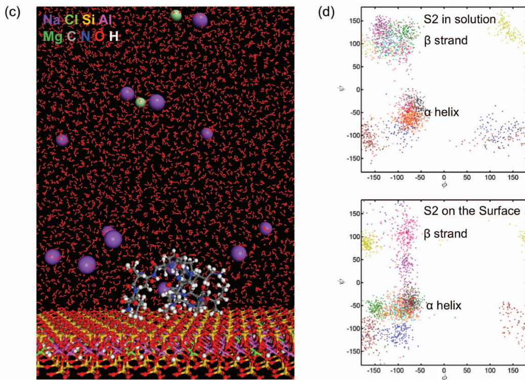
FIG. 14. (a) Peptides attracted to montmorillonite (CEC 91 meq/100 g) using phage display. Peptide S2 contains two cationic Lys side chains and is a very strong binder that can hardly be removed by washing cycles at pH = 7 (Drummy et al. , 2010). (b) Adsorption of the peptide S2 involves a cation exchange mechanism supported by the high isoelectric point (pI) and molecular simulation. Adsorption of nonionic peptides such as CR31 involves hydrogen bonds (Ser, Tyr) and polar interactions with the negatively charged surface. (c) Snapshot of the aqueous interface of montmorillonite with bound peptide S2 in atomistic simulation. Many sodium ions dissociate several nanometres away from the montmorillonite surface, consistent with swelling properties. The peptide replaces sodium ions near the surface and the formation of two Na^+ \cdots Cl^- ion pairs in the upper portion of the image can be seen. (Simulations involved montmorillonite (CEC 91 meq/100 g), 4000 water molecules, one peptide molecule, and the CVFF-PFF force field for 10 ns.) (d) Ramachandran plots for peptide S2 indicate \alpha helical and \beta strand conformational features in solution and on the surface, whereby the amount of helix and random coil dominate on the surface. The plot is specific for this peptide with multiple surface-binding groups.
