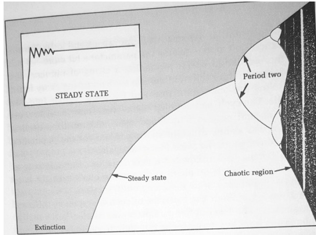
Figure 1 – Chaos
