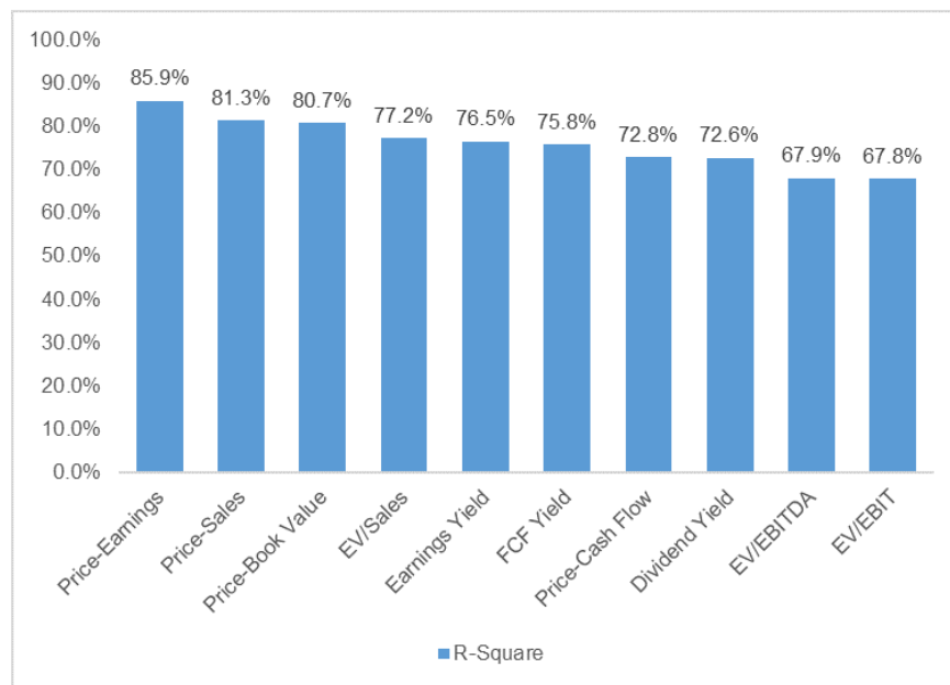
Figure 7.10.3: Comparative study of R^2 different regression obtained using different valuation metric on monthly data from Feb 2000 to April 2016. (Only the metrics that had a p -value < 0.05 for their coefficient are shown here)
