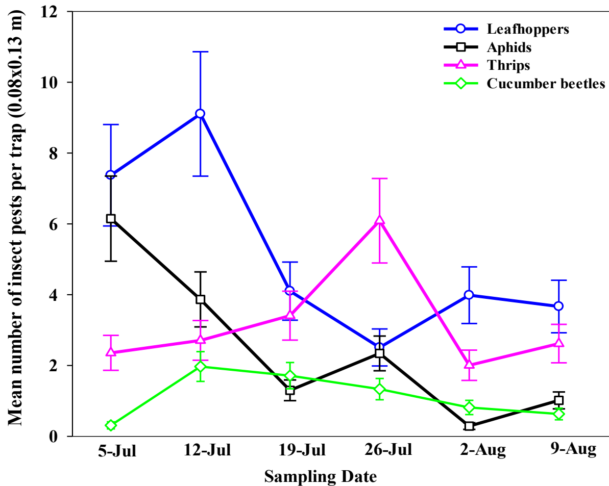
Figure 2: Mean ( \pm SE) number insect pests captured on the yellow sticky card traps by sampling dates in North Carolina.
