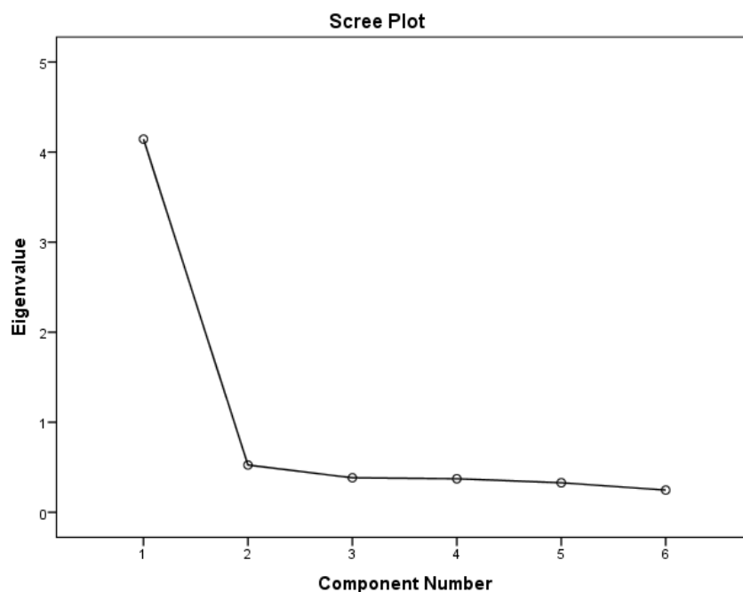
Figure 1. Scree plot used to visually suggest the number of factors to retain.
